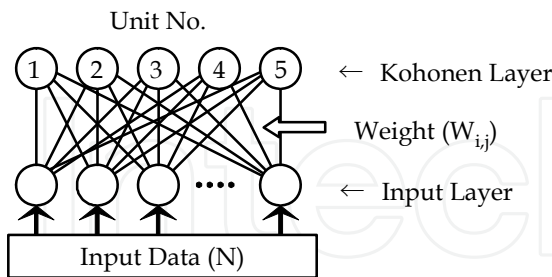
(a) Structure of SOM.
