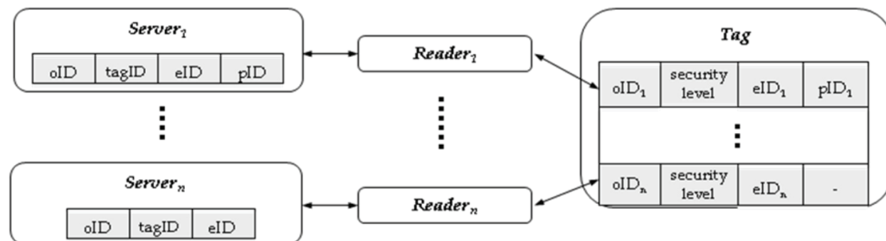
Fig. 2. Proposed multiple objects tag structure
