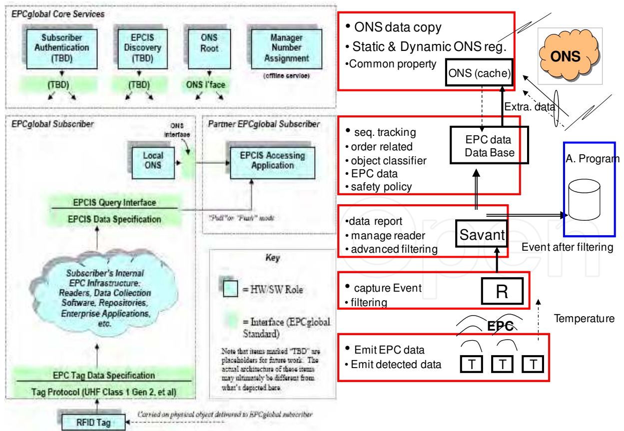
Fig. 3-4. A typical EPCglobal System Architecture
