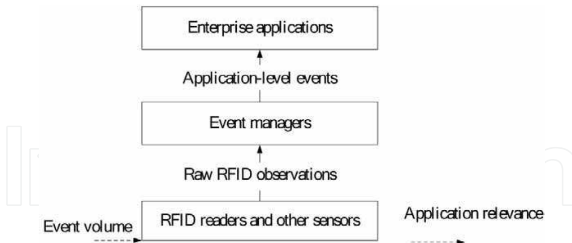
Fig. 2-7. Event volume and relevance through different layers of an RFID system
