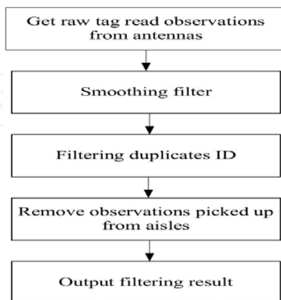
Fig. 2-5. Procedure of Filtering the Events
