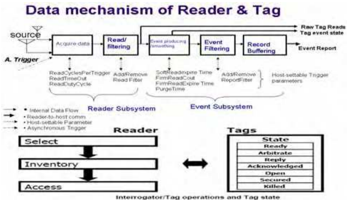
Fig. 2-6. The Data mechanism of reader and tag
