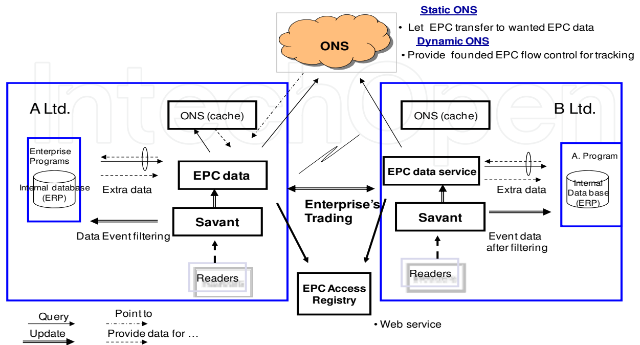
Fig. 3-5. The EPCglobal Network architecture between enterprises
