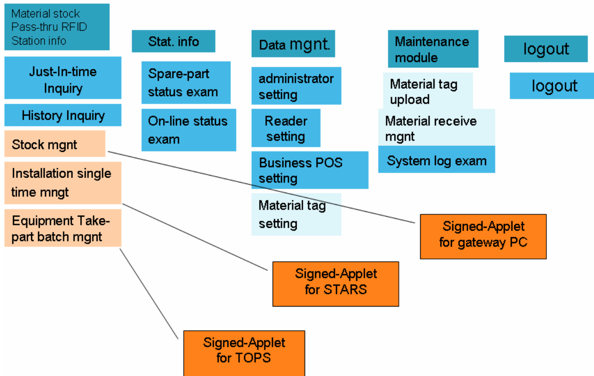
Fig. 4-3. The Functional Structure of RamMIS Website.
