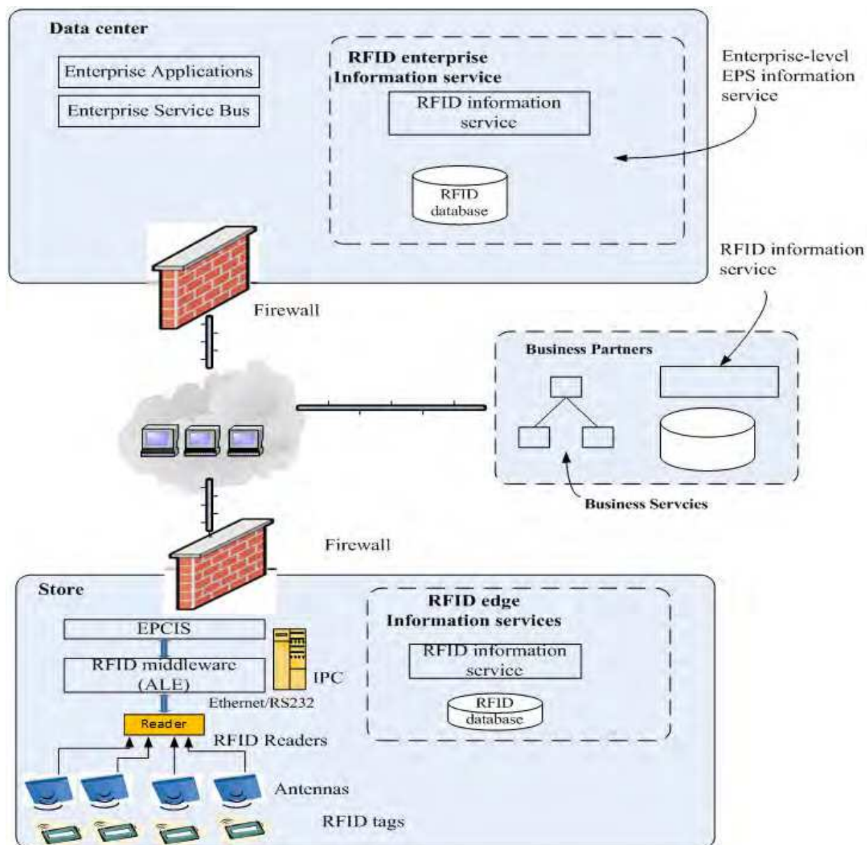
Fig. 2-2. RFID System Architecture
