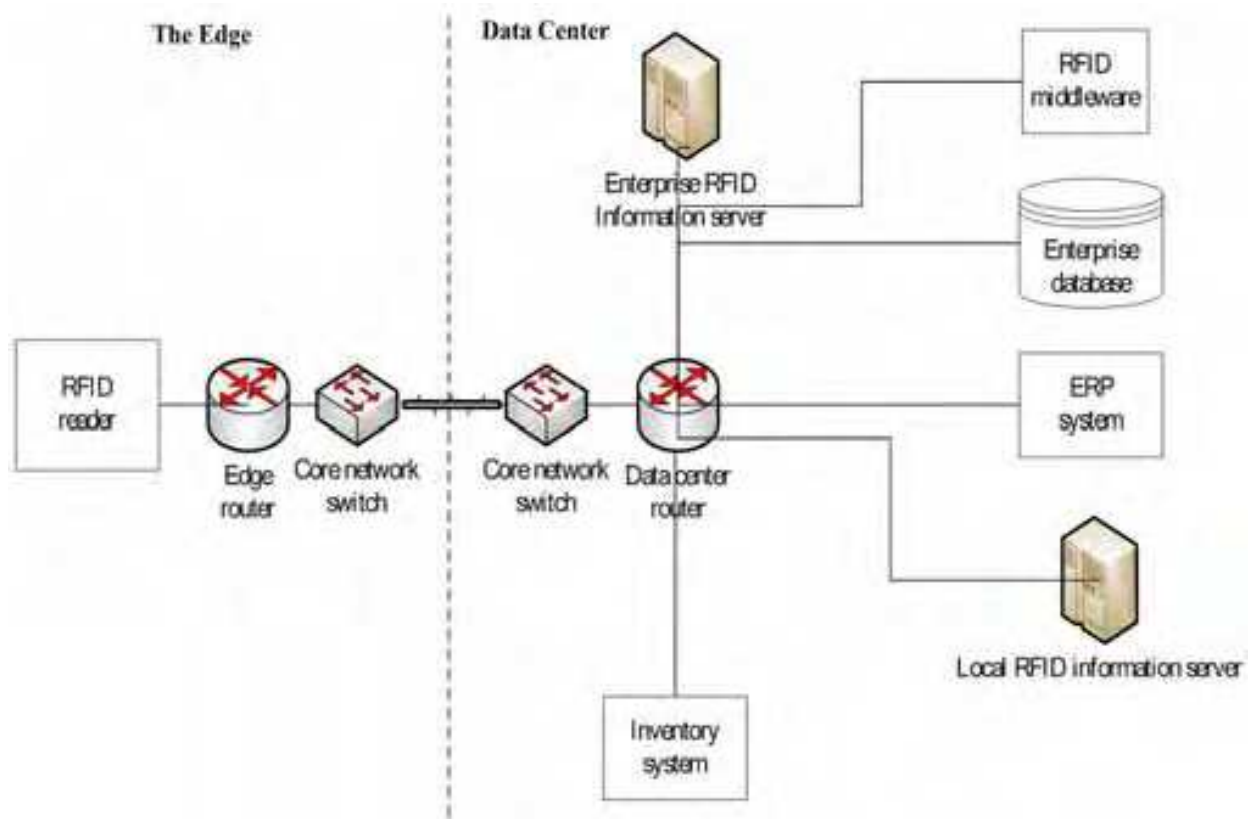
Fig. 3-6. The centralized approach
