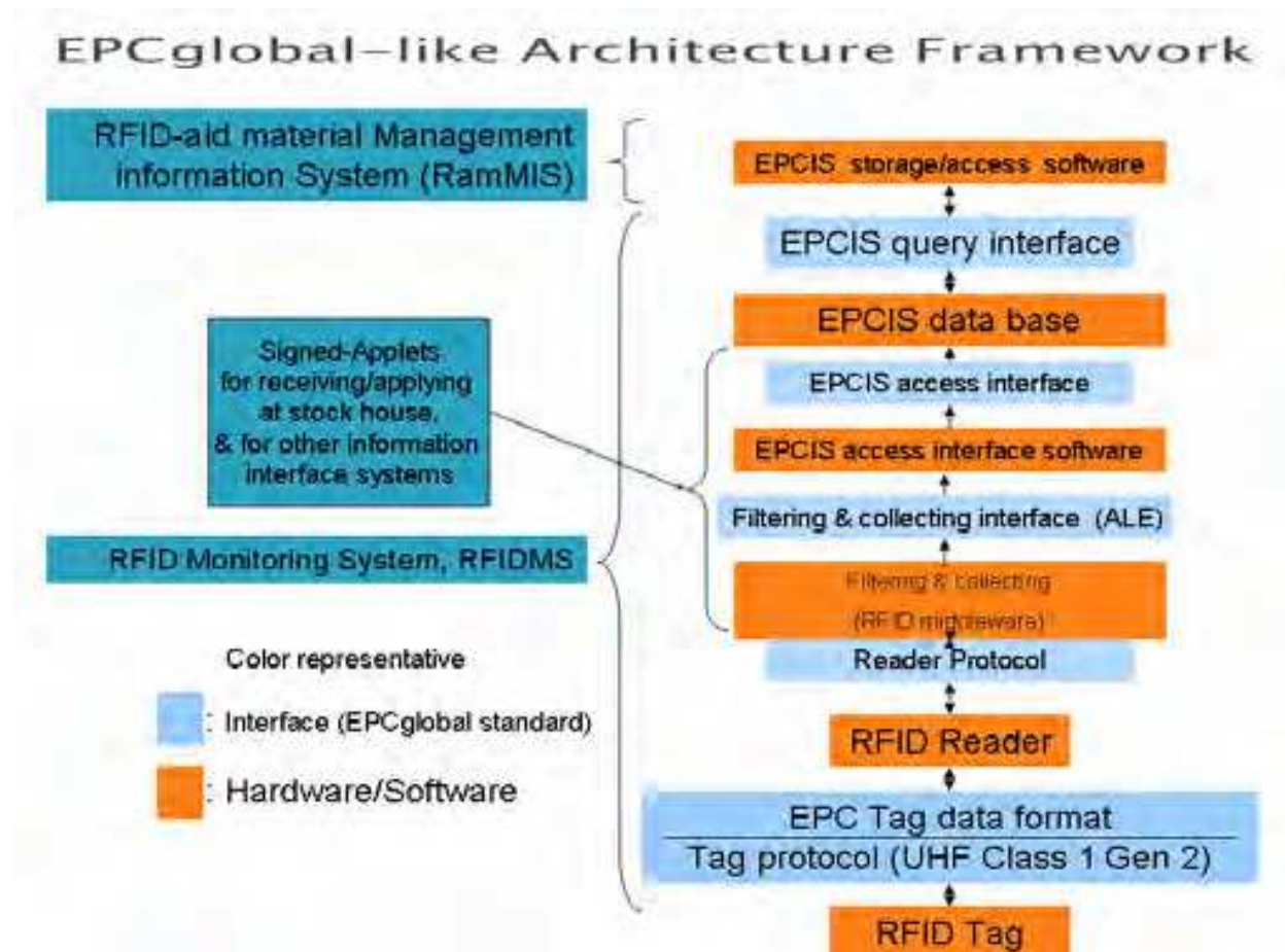
Fig. 4-2. EPCglobal-like Architecture Framework
