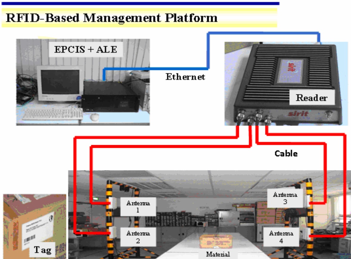
Fig. 2-3. the implementation of RFID-Based Management Platform
