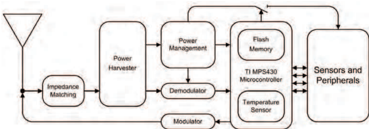
Fig. 3. Block Diagram of the WISP
