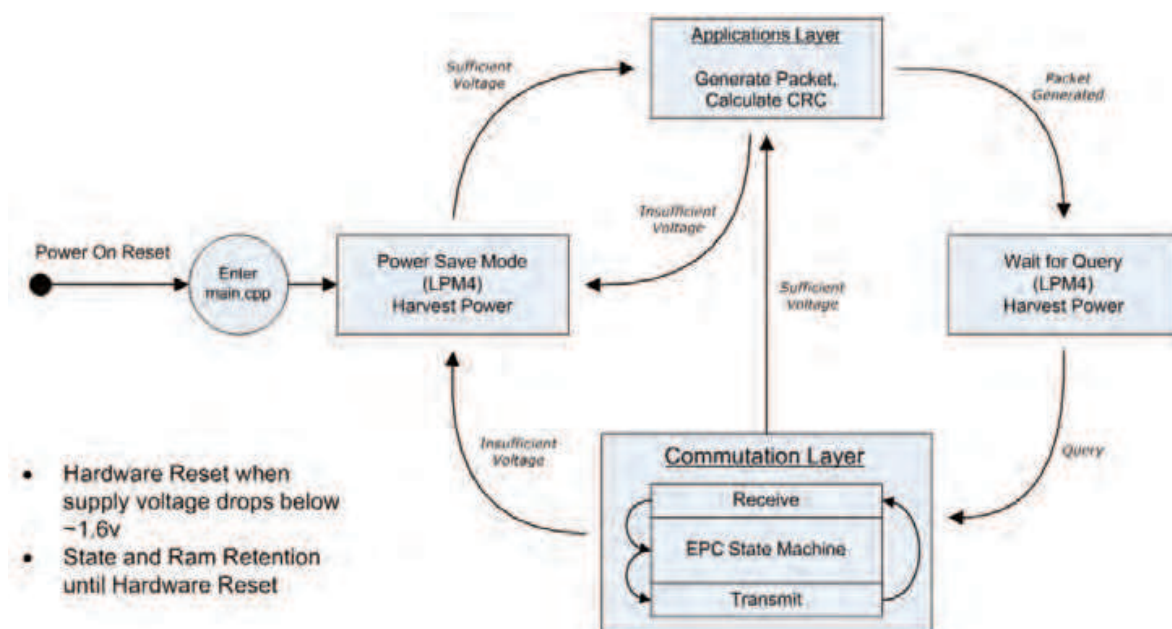
Fig. 5. Power Management Algorithm
