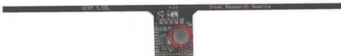
Fig. 7. WISP data logger with operational Super capacitor
