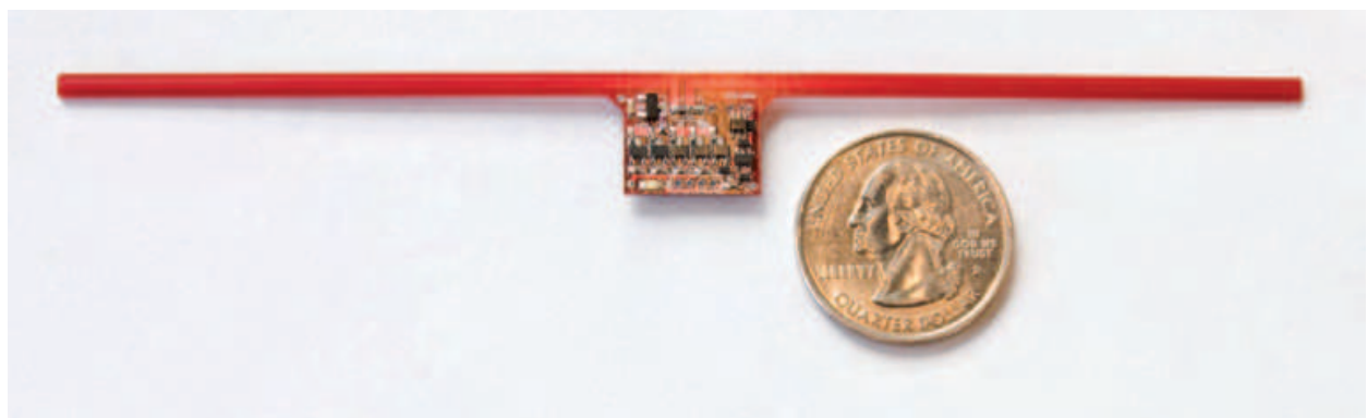
Fig. 2. Wireless Identification and Sensing Platform (WISP)
