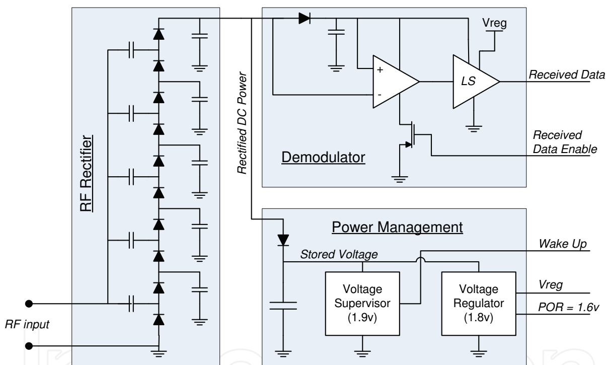
Fig. 4. Schematic of the Analog Front End
