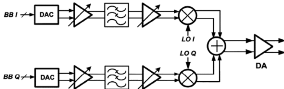
Fig. 18. Transmitter architecture
