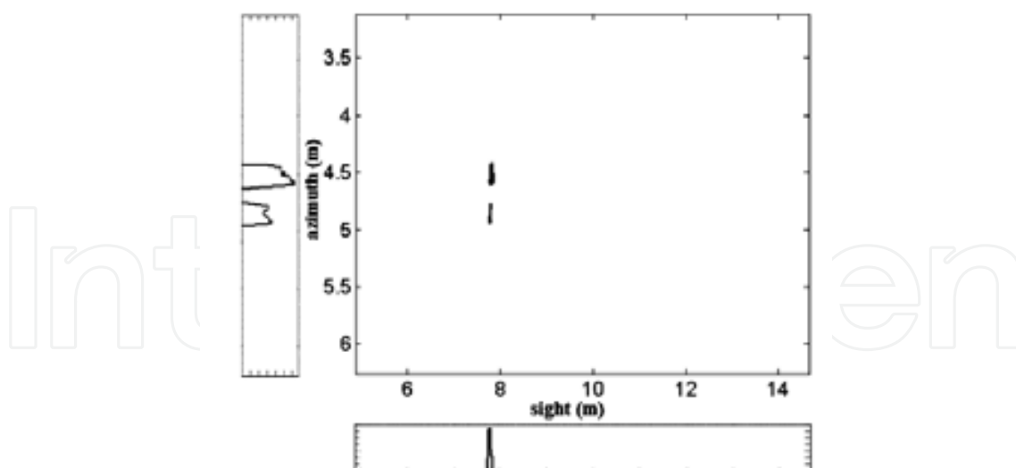
Fig. 12. Segmented SAS image and repartition of the segmented pixels according to the two axes. Computed entropies: X-axis: 3.46; Y-axis: 4.58
