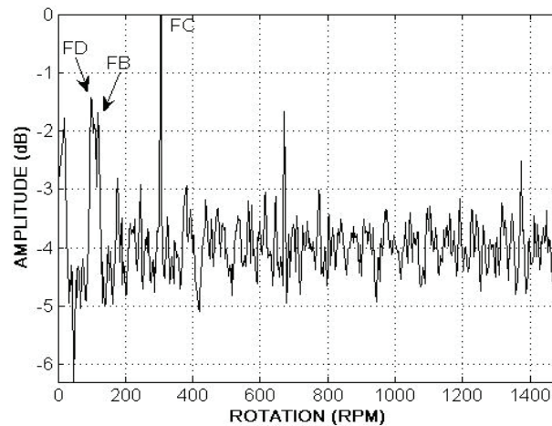
Fig. 12. DEMON analysis at 076^\circ .
