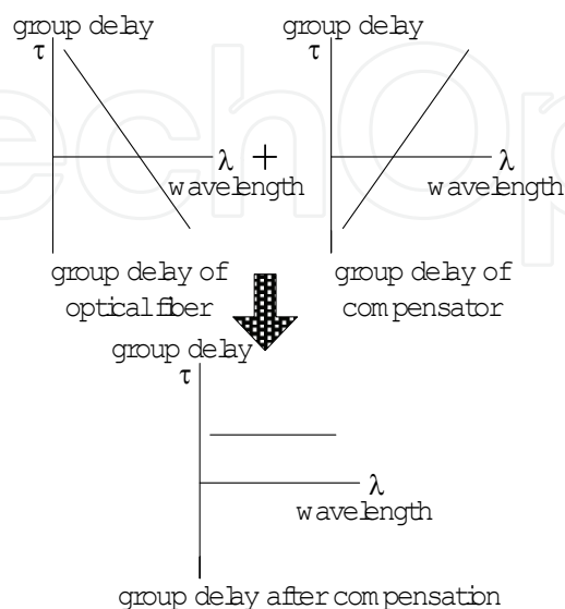
Fig. 5. Principle of chromatic dispersion compensation.
