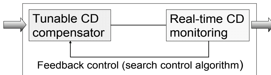
Fig. 1. Adaptive CD compensation in the receiver.
