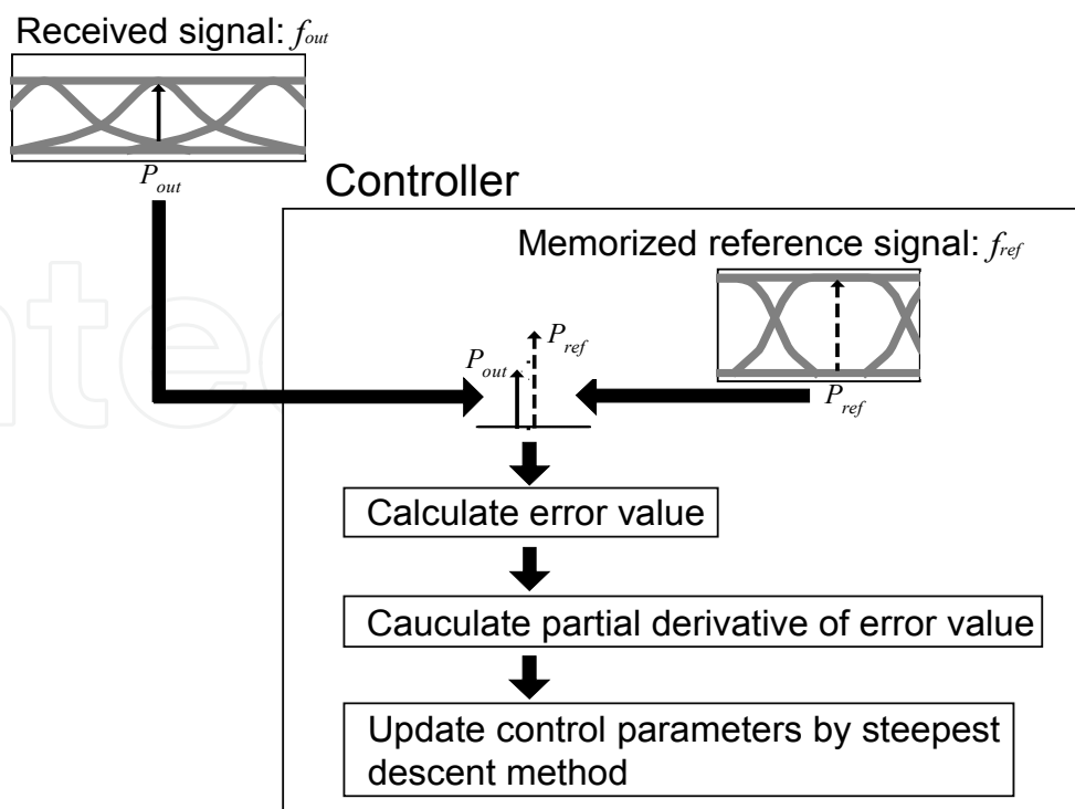
Fig. 7. Procedure of proposed steepest-descent-based control.
