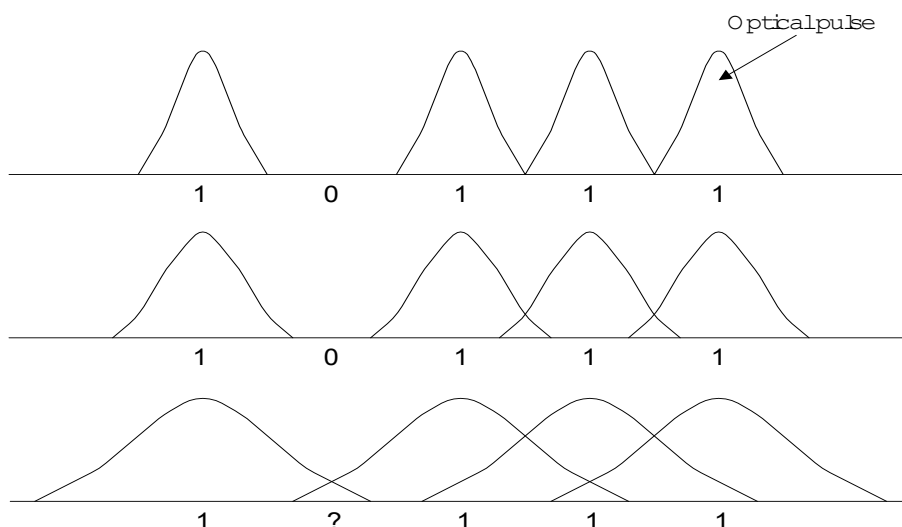
Fig. 4. Interference of neighboring pulses in optical communication.
