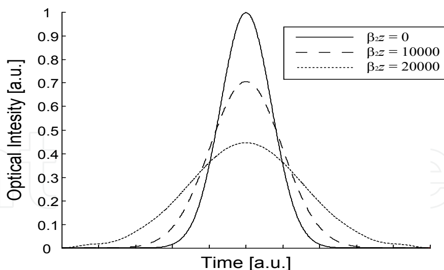
Fig. 3. Optical pulses affected by chromatic dispersion.
