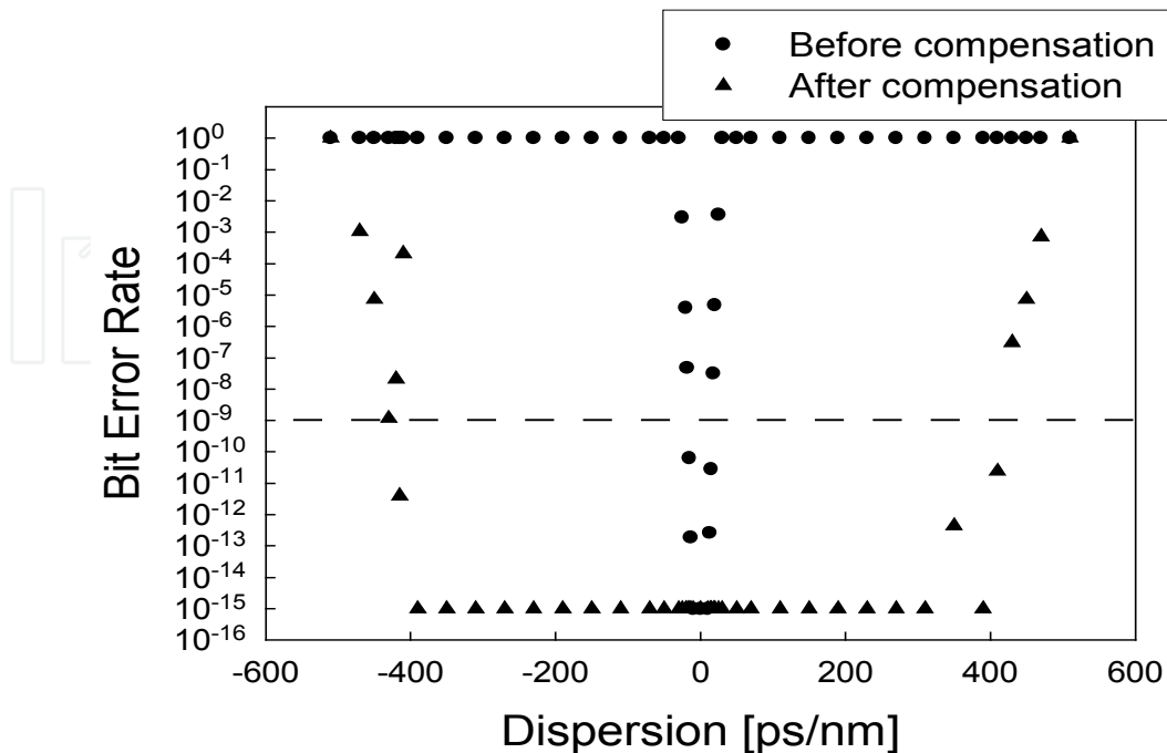
Fig. 10. Compensation range of the proposed method at 40 Gb/s.
