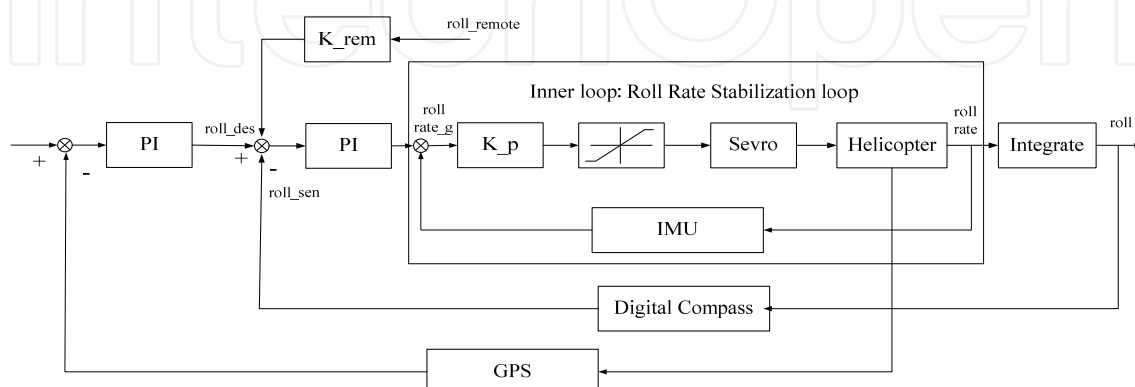
Figure 18. Roll control scheme
