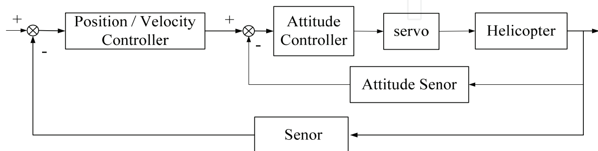
Figure 14. Overall flight control scheme
