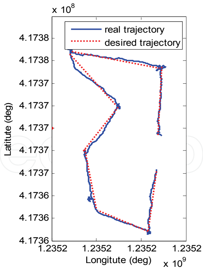
Figure 22. Desired and real trajectory
