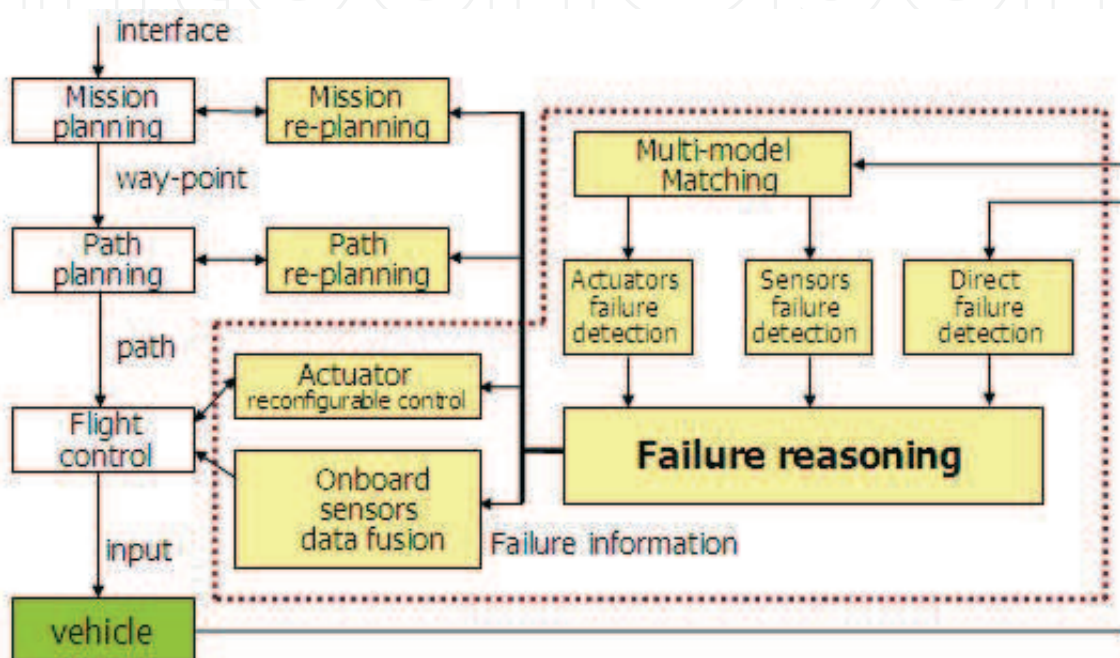
Figure 23. Overall flight control scheme
