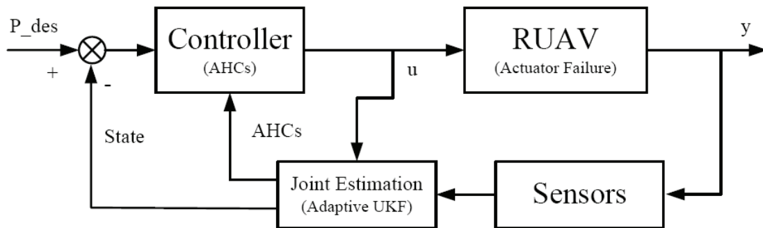
Figure 26. Actuator fault tolerant control scheme
