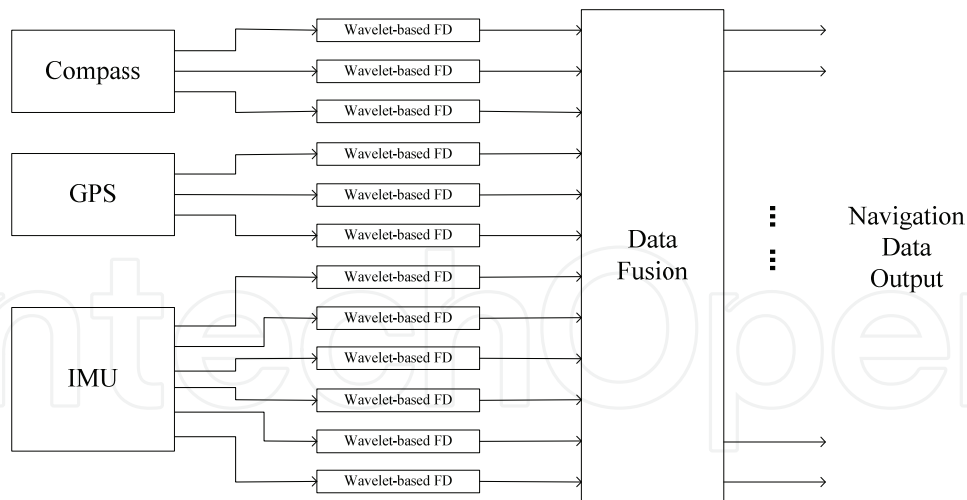
Figure 24. Wavelet-transform based sensors failure detection
