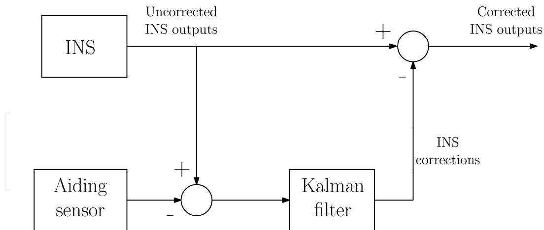
Figure 8. Complementary filtering as used for INS aiding
