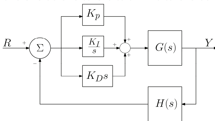
Figure 11. A PID controller
