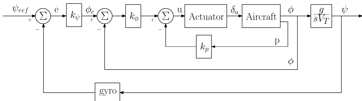
Figure 10. Classical heading hold autopilot system
