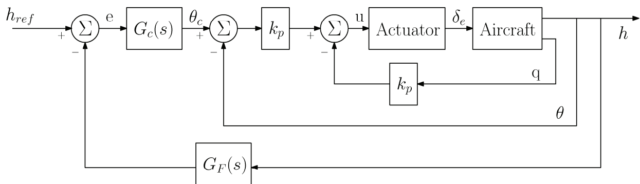
Figure 9. Classical altitude hold autopilot system
