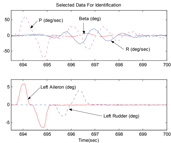
Figure 6. Flight Data for Linear Model Identification
