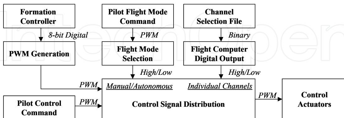
Figure 5. Control Signal Distribution System
