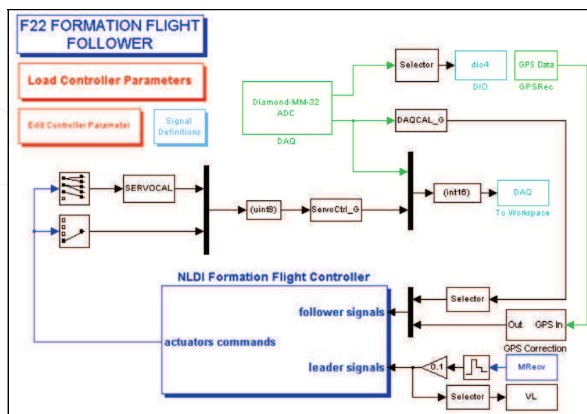
Figure12. Simulink Diagram of the 'Follower' Aircraft Software
