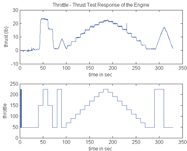
Figure 10. Throttle Thrust Response in Test Time Sequence
