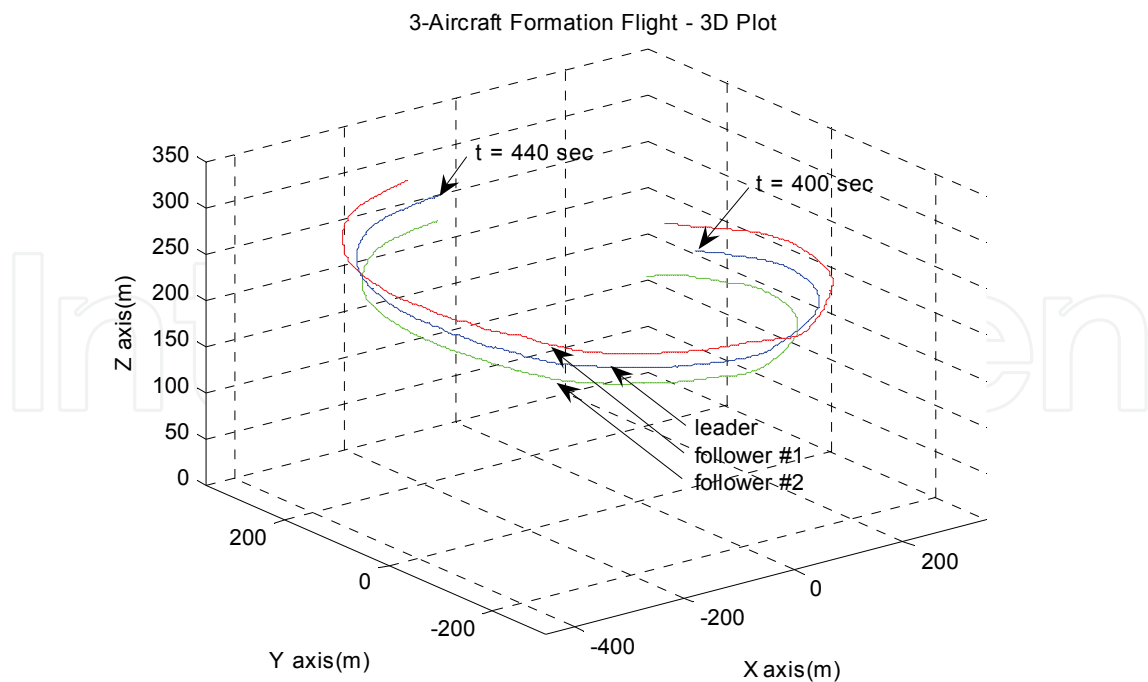
Figure 16. 3- Aircraft Formation Test - 3D Trajectory (Blue='leader', Red=Outside 'follower', Green=Inside 'follower')
