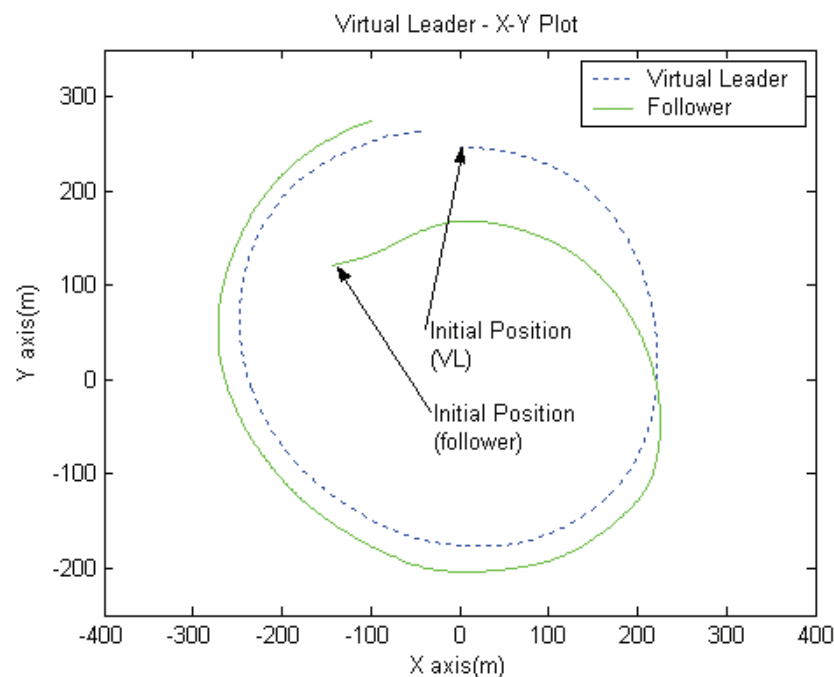
Figure 14. 'Virtual leader' Test - X-Y Plane
