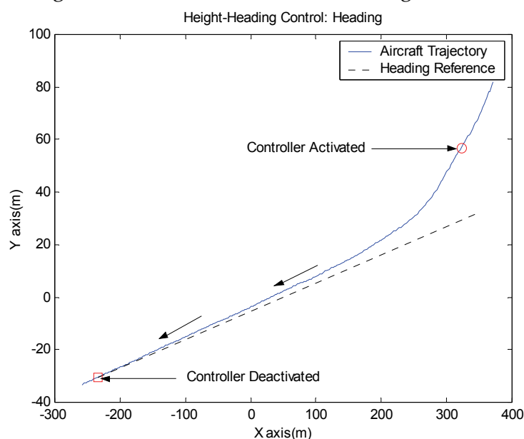
Figure 13. Heading Control Experiment
