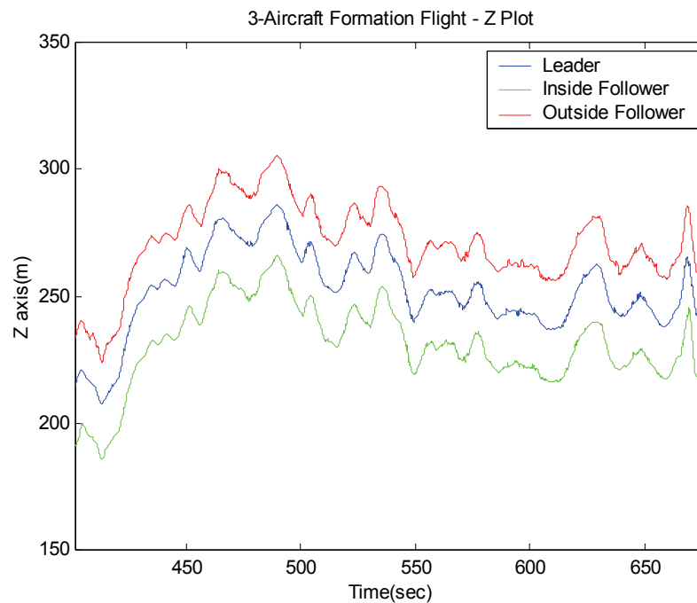
Figure 17. 3-Aircraft Formation Test - Altitude
