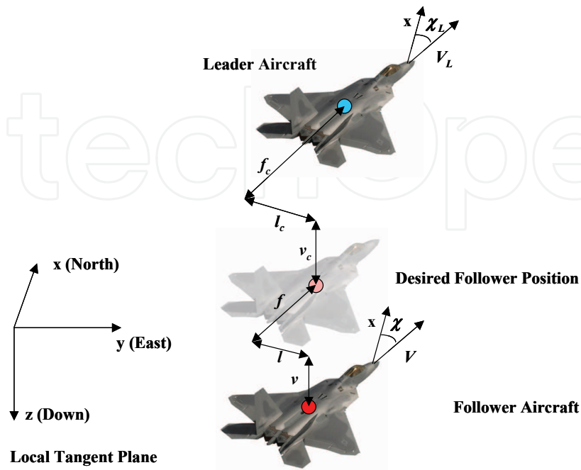
Figure 1. Formation Geometry
