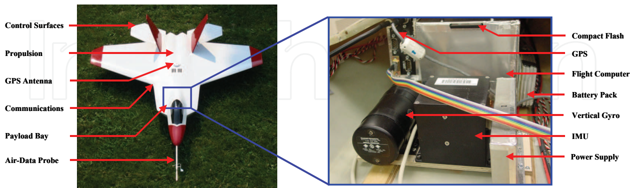
Figure 4. 'Follower' Aircraft and Avionics System
