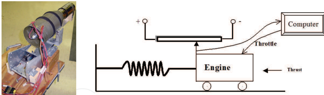
Figure 9. Engine Ground Test Setup and Schematic
