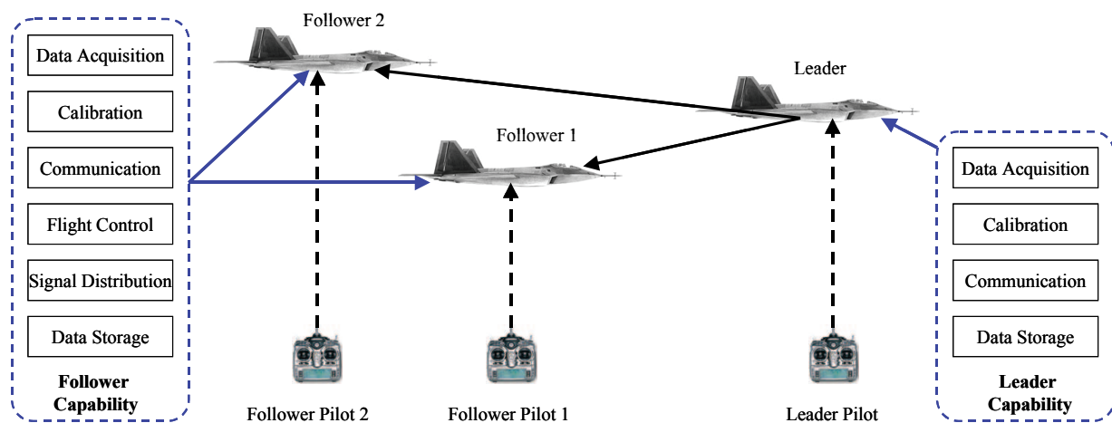
Figure 3. Formation Configuration and Capabilities
