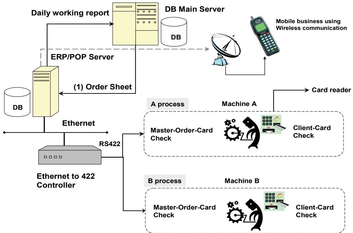
Fig. 1. Architecture of system for the parts
