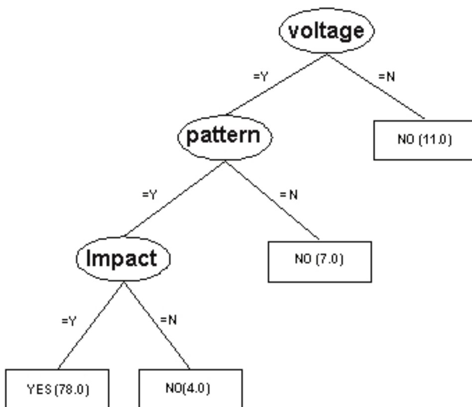
Fig. 6. Application of C4.5 algorithm to LCD line
