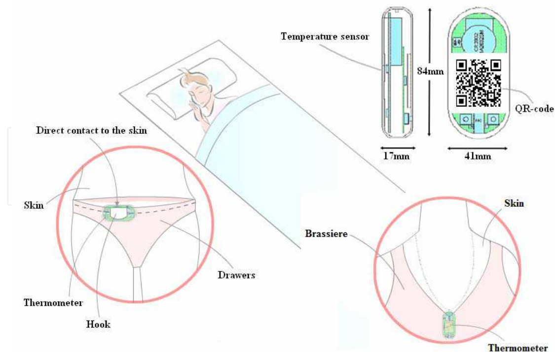
Fig. 8. A small, light wearable device (size = 41 \times 84 \times 17 mm 3 , weight = 59 g) for cutaneous temperature measurements during sleep (QOL Co. Ltd., 2008).
