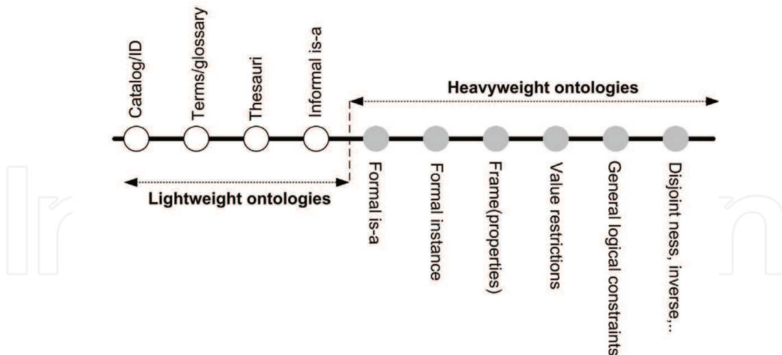
Fig. 1. An Ontology Expressiveness Spectrum adapted from McGuinness (2003)
