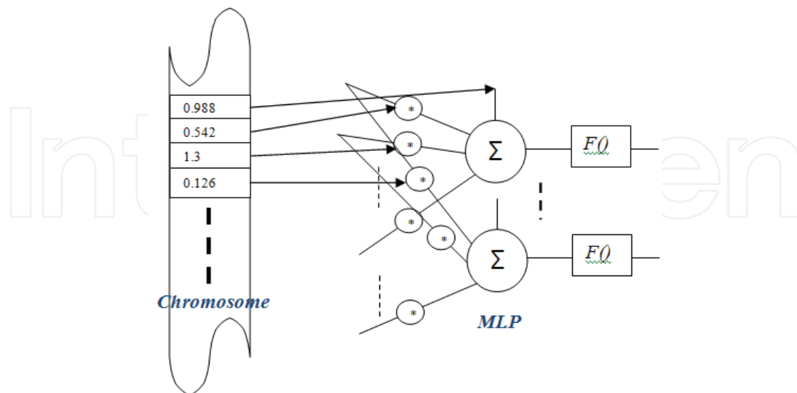
Fig. 8. Weight/bias mapping
