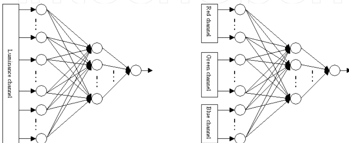
Fig. 6. Conventional v.s. proposed MLNN structures
