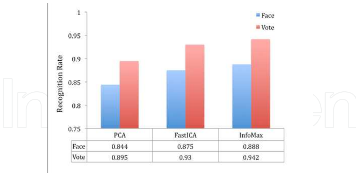
Fig. 7. Face and VOTE performance.
