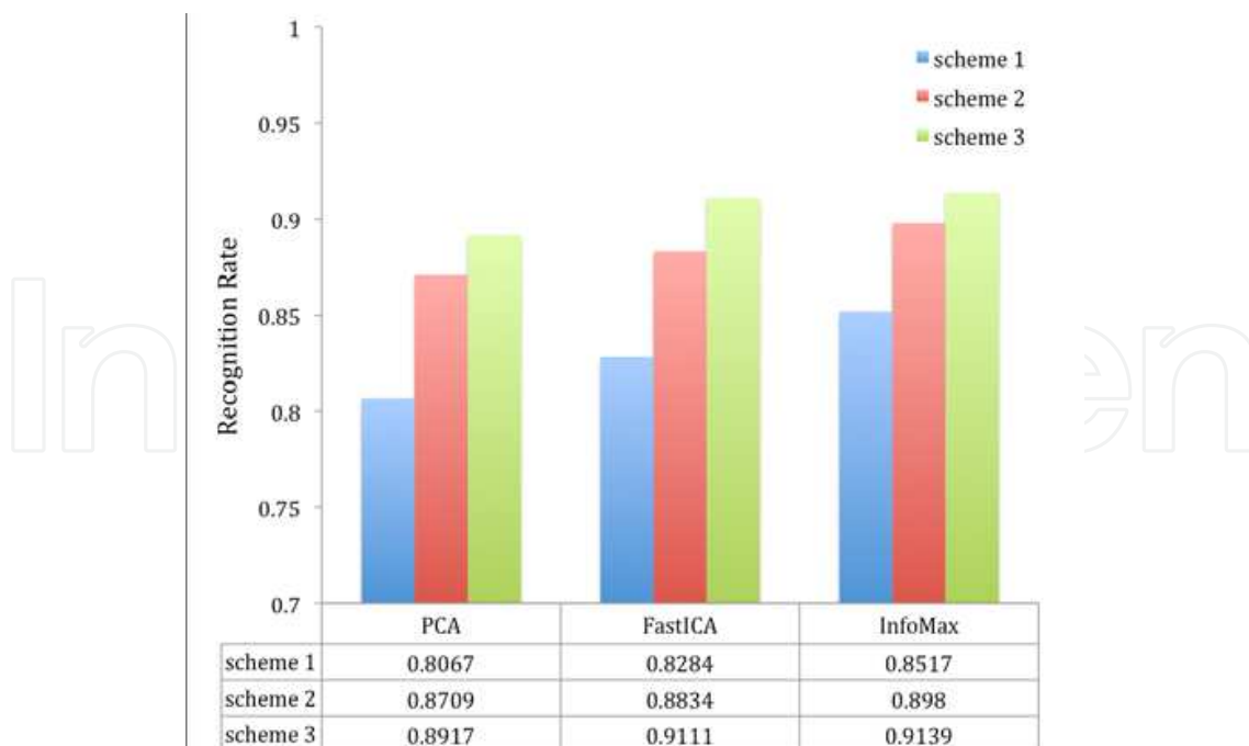
Fig. 5. Comparison of the three algorithms PCA, FastICA, and InfoMax.
