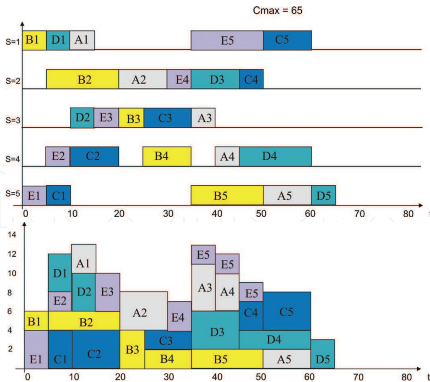
Fig. 11. Gantt's charts for answer to the question implemented in predicate opc\_g(\_, \_) , C_{max}^*=65, L=14 (Example_1b).
