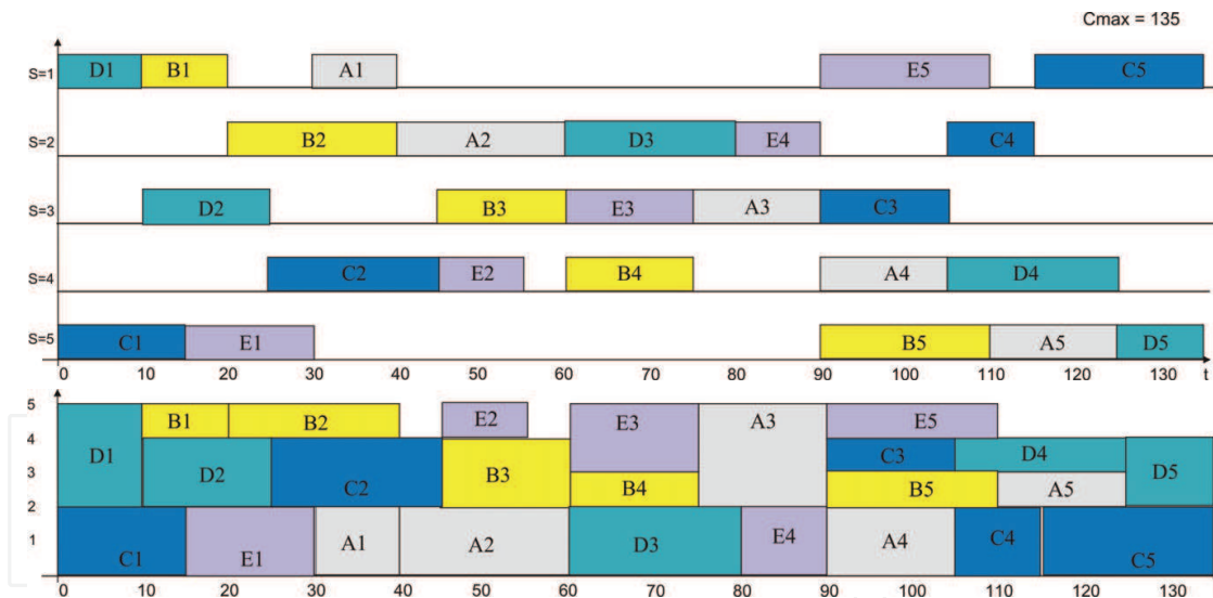
Fig. 9. Gantt's charts for the answer to the question implemented in predicate opc_g(5,_) , C_{max}^*=135 , L=5 (Example_1a).
