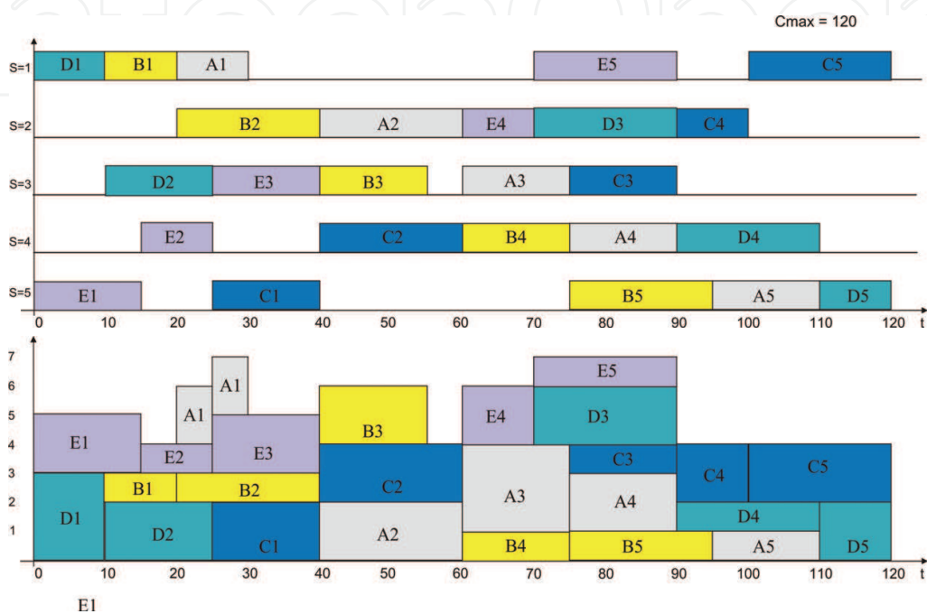
Fig. 5. Gantt’s charts for the answer to the question implemented in predicate opc\_g(\_,\_) , C_{max}^*=120, L=7 (Example_1a).
