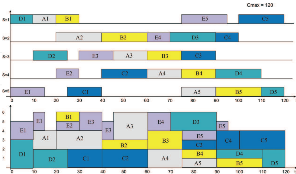
Fig. 6. Gantt’s charts for the answer to the question implemented in predicate opc\_d(\_, 120) , L_{min}=6, C_{max}= C_{max}^*=120 (Example_1a).
