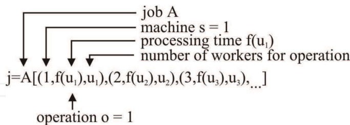
Fig. 4b. Description of task (job) data structure for job-shop computational example (Example_1b) – the processing times depend on allocated number of workers.
