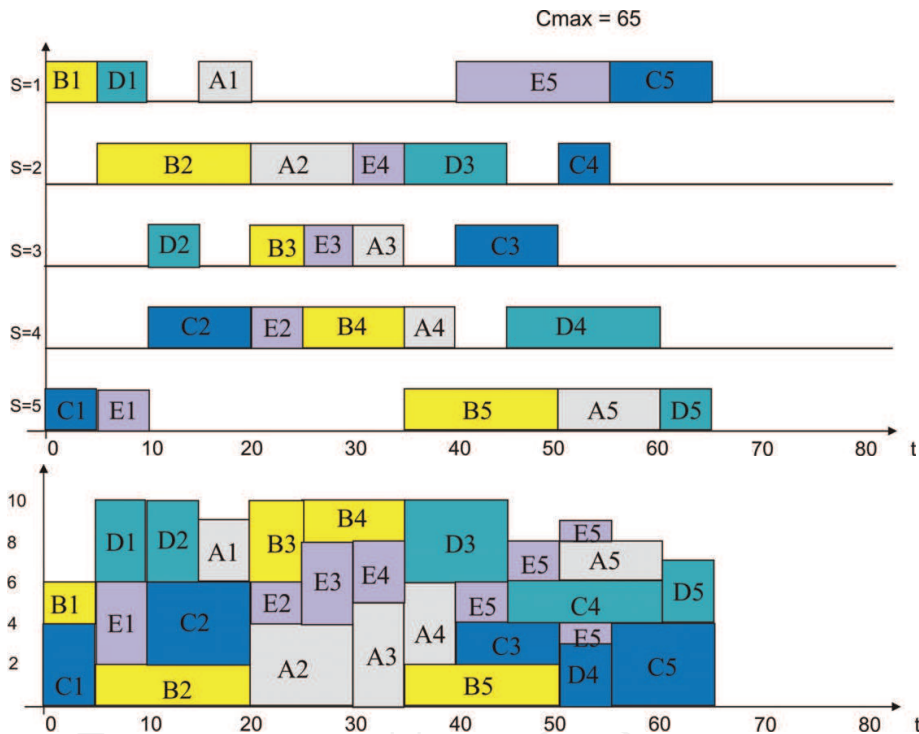
Fig. 13. Gantt's charts for answer to the question implemented in predicate opc_d(_,65) , L_{min}=10, C_{max}=C_{max}^*=65 (Example_1b).
