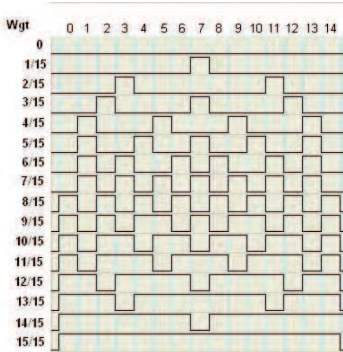
Fig. 8. The first fifteen weights in the proposed system
