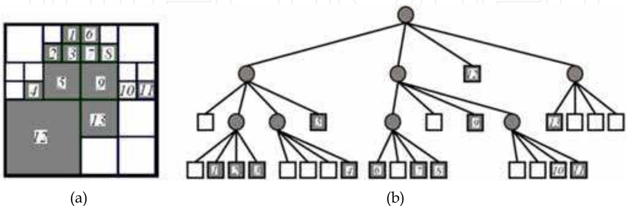
Fig. 15. Adaptive resolution representations (a) Adaptive Grid Resolution (AGR) image; (b) quad-tree decomposition of AGR. Due to the fact that the normalization before computing AGR, AGR representation is invariant under rotation, scaling and translation. It is also computationally simple.
