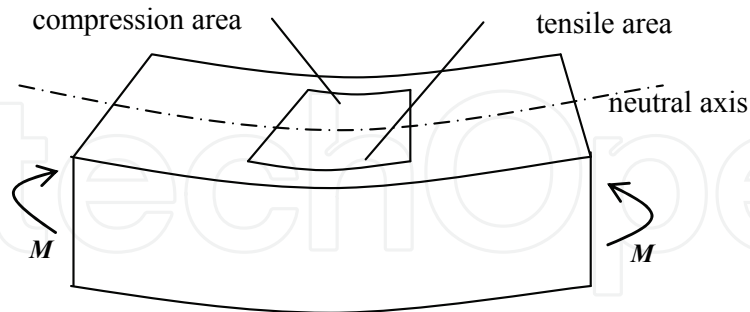
Fig. 9. The beam is under bending moment in its flank
