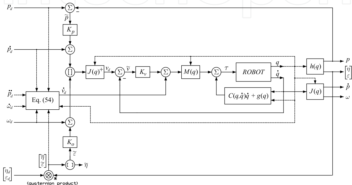
Figure 6. Hierarchical control: RMRC + inverse-dynamics velocity controller
