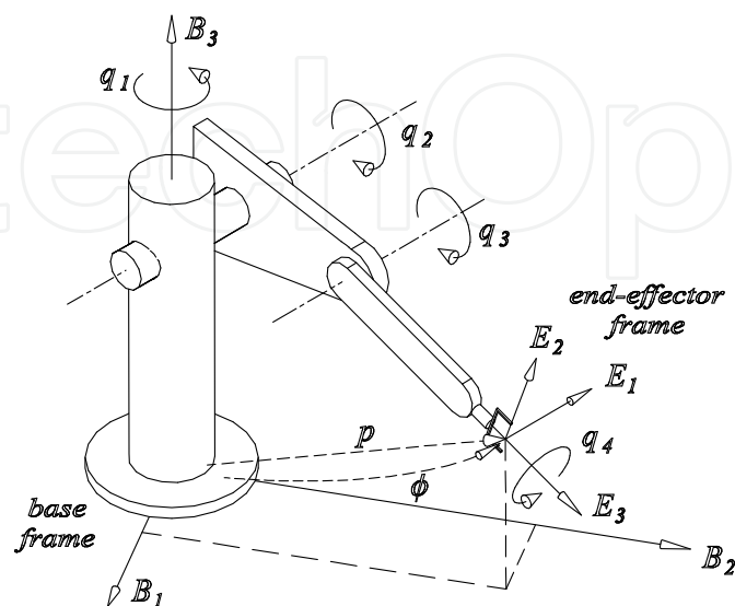
Figure 3. A 4-dof serial robot manipulator
