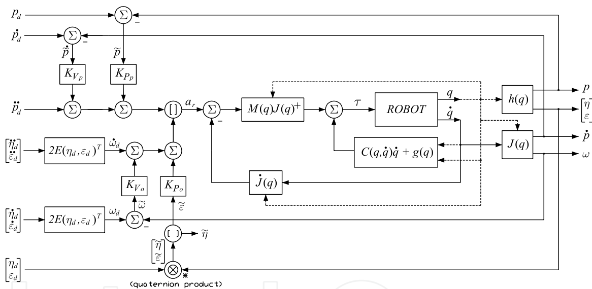
Figure 7. Resolved acceleration product controller with Euler parameters
