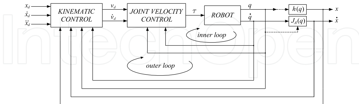
Figure 4. Pose-space hierarchical control
