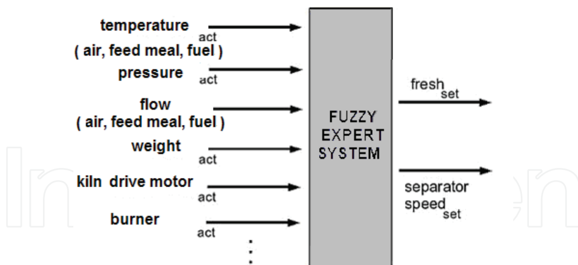
Fig. 20. Fuzzy-Expert system
