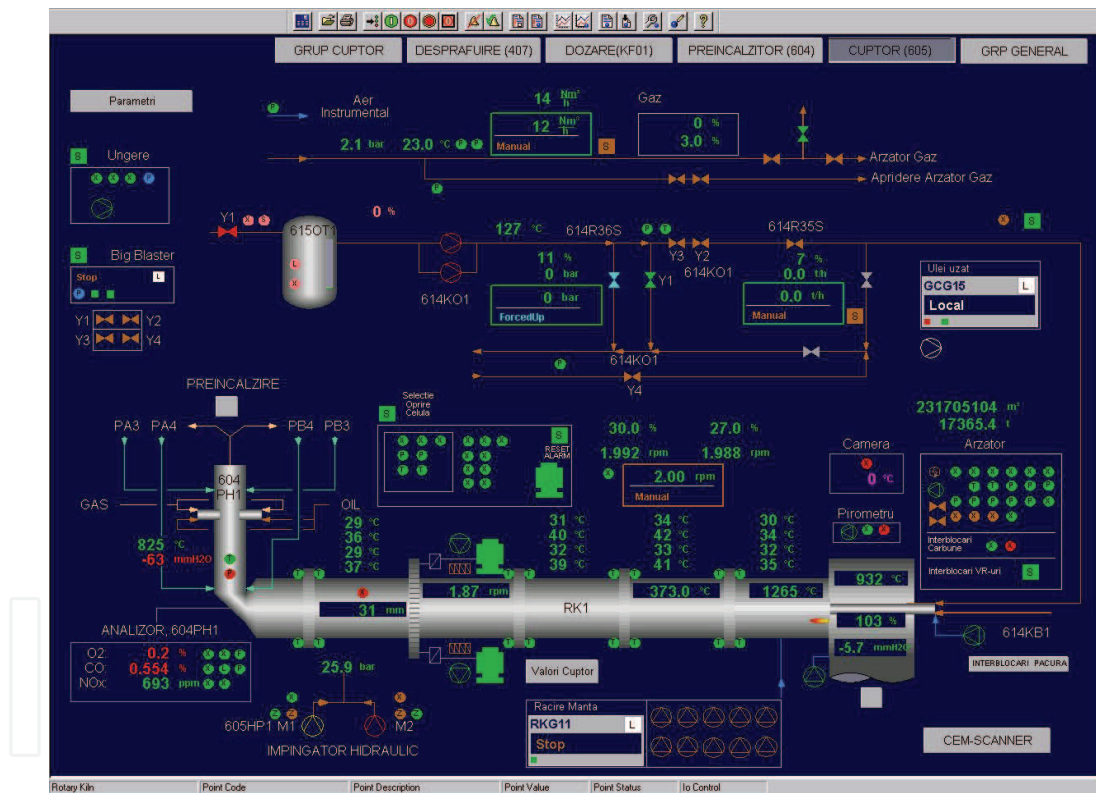
Fig. 18. Monitoring system and control kiln
