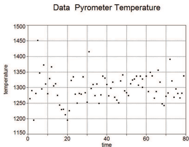
Fig. 12. Pyrometer temperature
