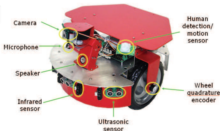
Fig. 9. Wireless Mobile Robot
