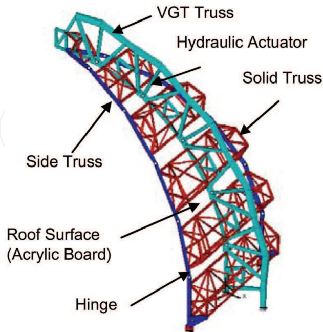
Fig. 12. Roof Structure Installed on VGT Mechanism
