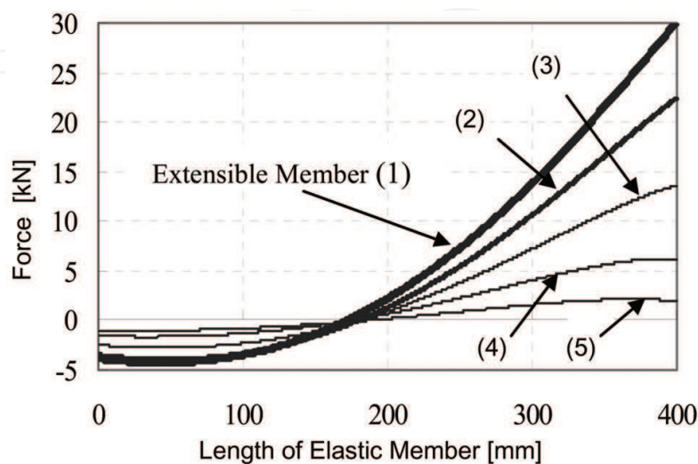
Fig. 10. Dynamical Force Acted on Extensible Member
