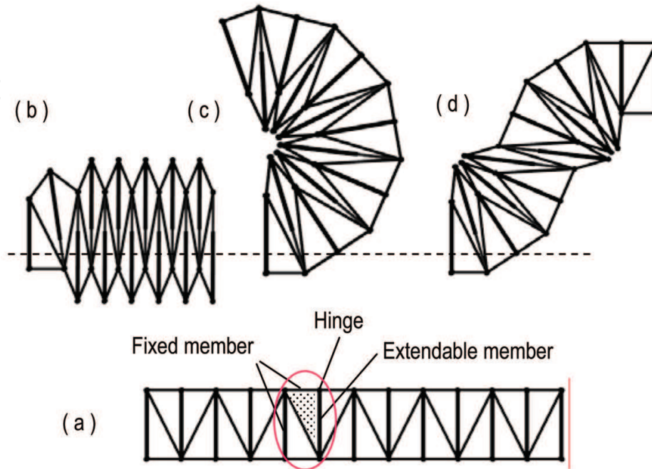
Fig. 2. Transformation of Beam Shape Using VGT
