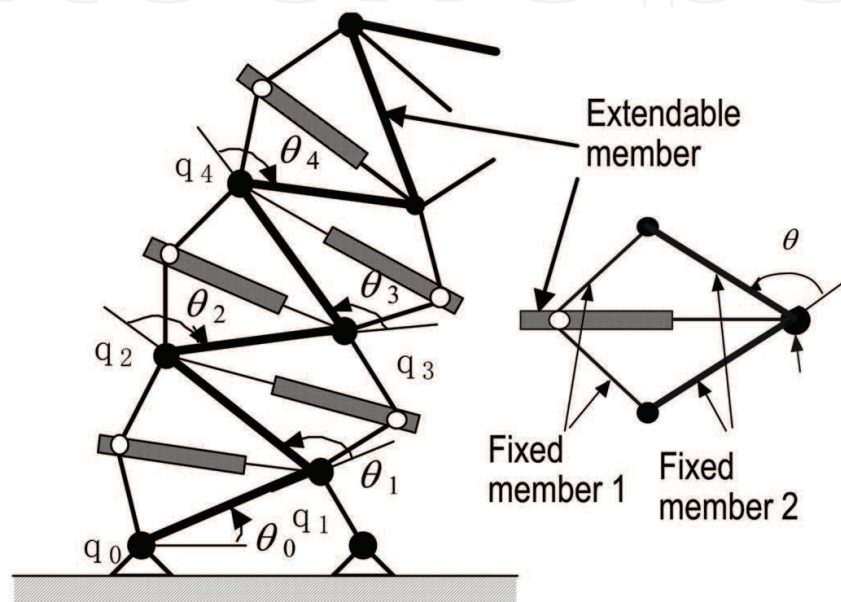
Fig. 3. Two- dimensional VGT Unit and Analysis Model
