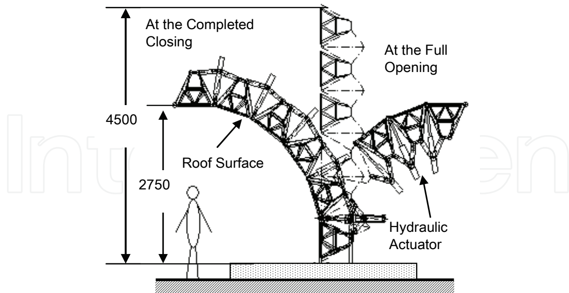
Fig. 13. Schematic Structure of a Reduced Model of Flowering Dome
