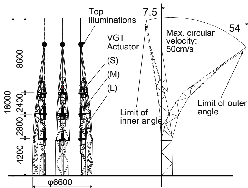
Fig. 17. Arrangement of VGT Actuator and the Movement Range of Tower
