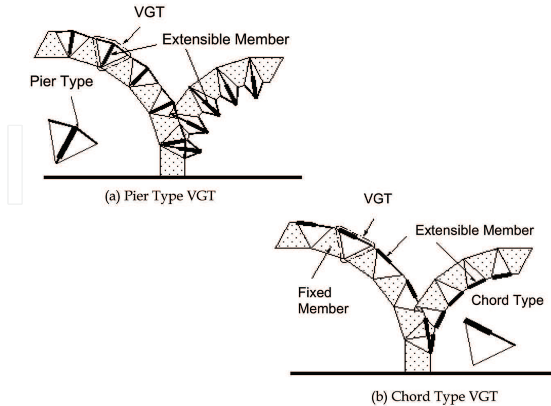
Fig. 7. Composition Type of VGT Arrangement
