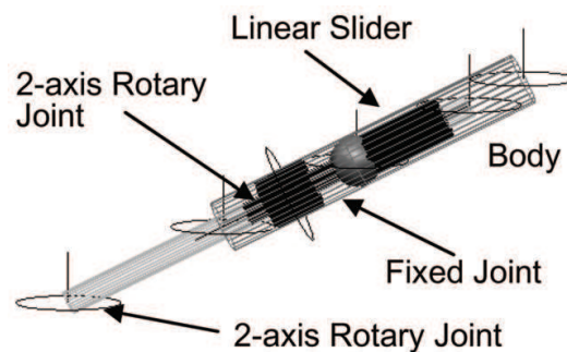
Fig. 9. A Model of an Extensible Member in Dynamic Software
