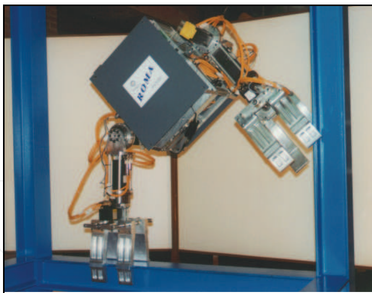
Fig. 6. ROMA climbing inspection robot
