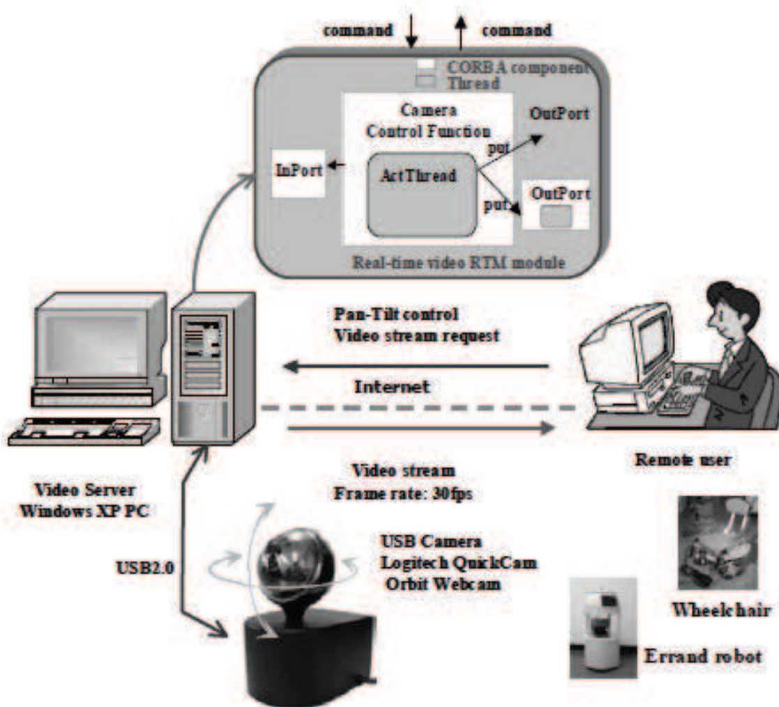
Fig. 12. Structure of RT video stream functional component.
