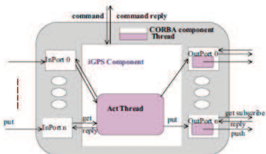
Fig.2. Structure of RT Component.
