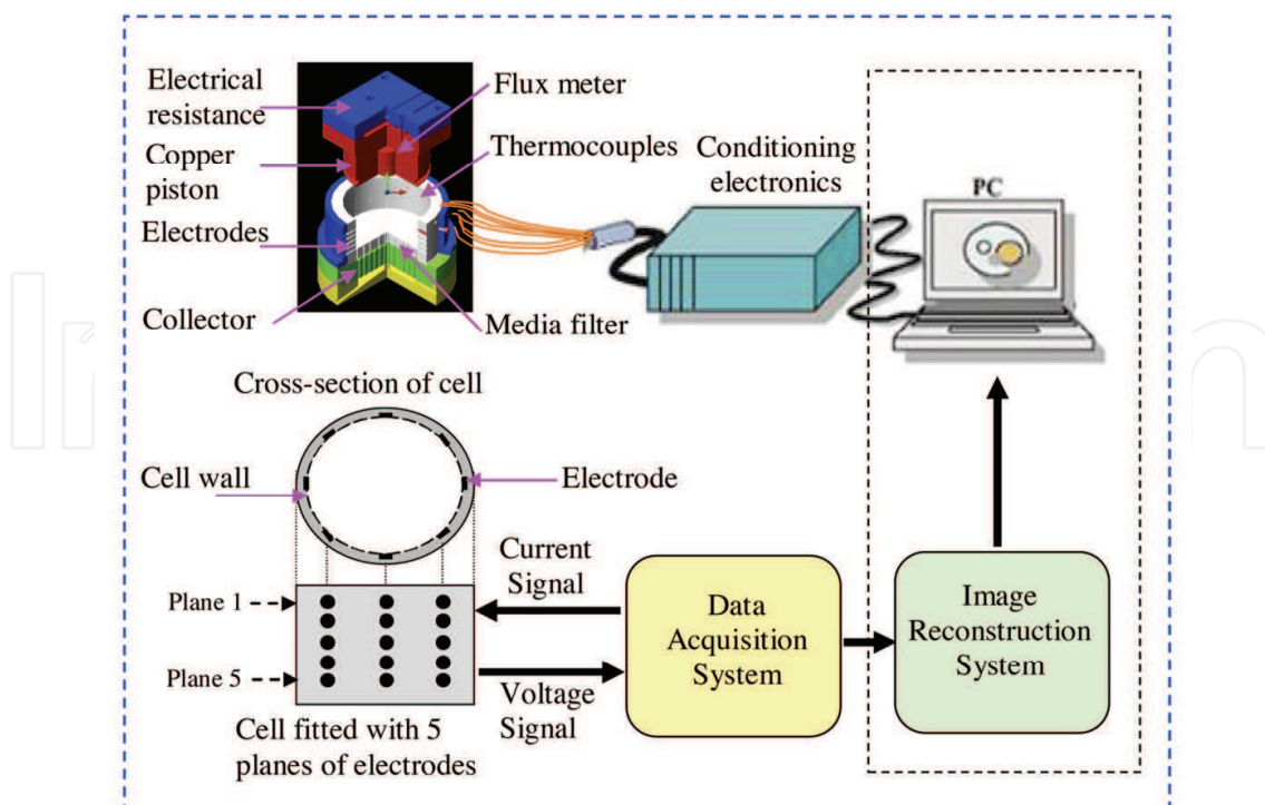
Figure 5. Schematic diagram of the measurement principle of ERT system
