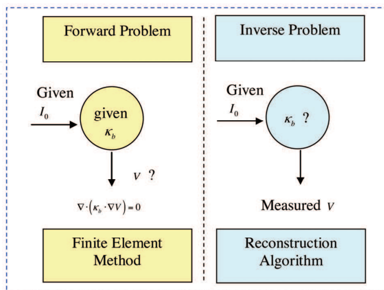
Figure 2. ERT forward and inverse problems
