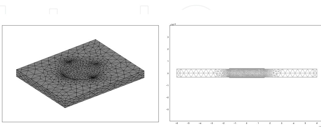
Figure 12. Simulation model for resonator using TE3 mode vibration
