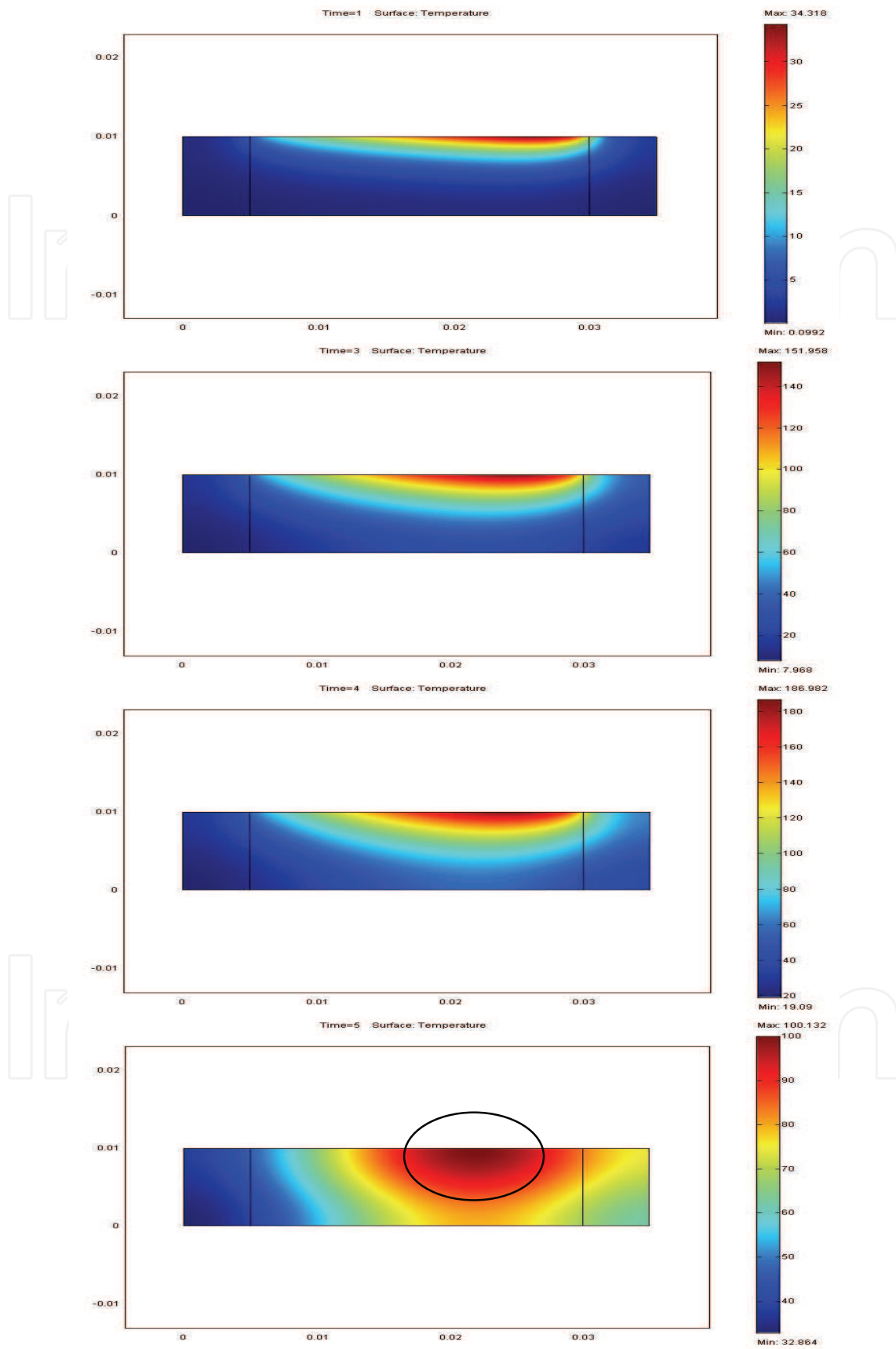
Figure 10. Change of the surface temperature across the disk brake, at time steps, 1, 3, 4, and 5s
