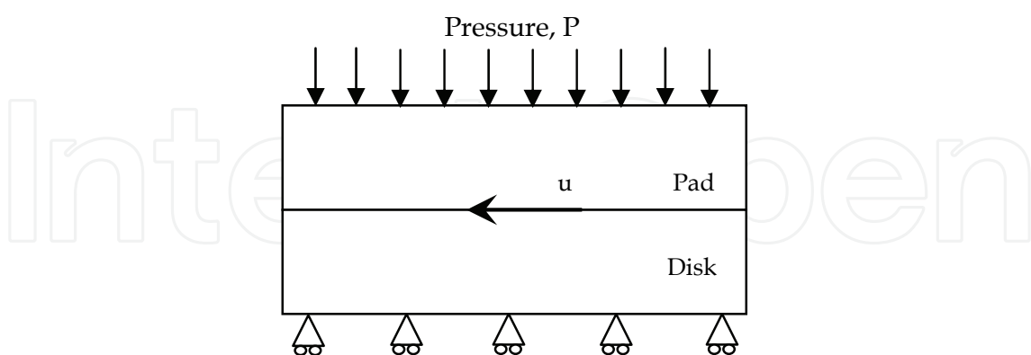
Figure 6. Elastic problem boundary conditions
