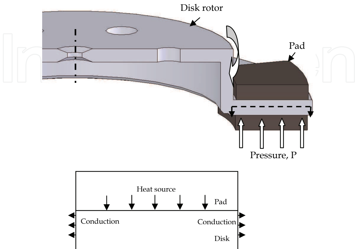
Figure 5. Heat transfer boundary conditions
