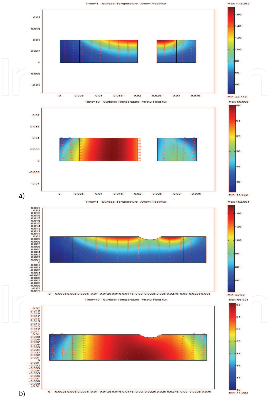
Figure 12. Comparison between the temperature distribution and the heat flux produce in a) the perforated disks b) the notched disks
