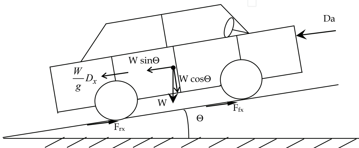
Figure 3. The major forces acting on the vehicle
