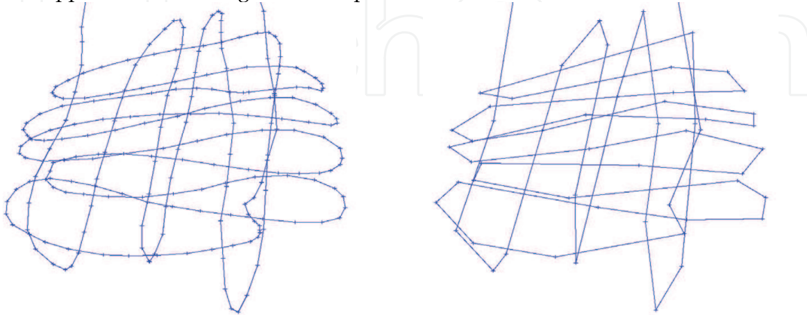
Figure 12. Scanline path for ultrasound recording of the human skull. Left: original path (307 path points), right: smoothed path using K_1 and d_{lim} = 1 mm (90 path points)
