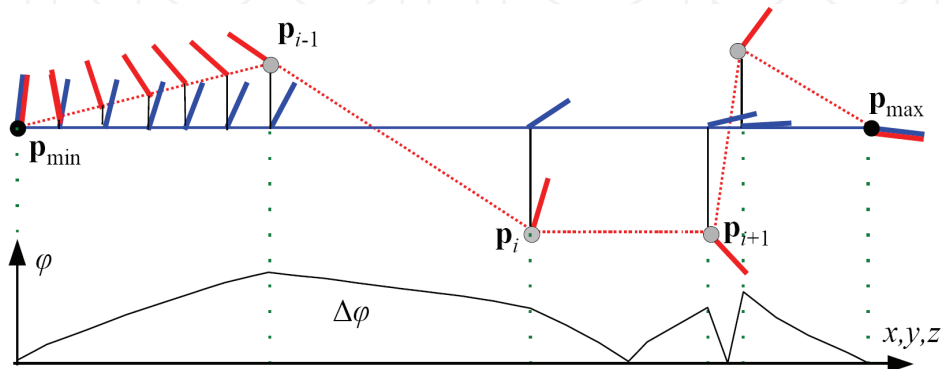
Figure 7. Sketch visualizing the computation of the angle sum \Delta\varphi . For simplification, the angle is represented only in 1D. Top: Curve progression of the orientation of a smoothed path [p_{\min}, p_{\max}] (blue) and the original path [p_{\min}, \dots, p_{i-1}, p_i, p_{i+1}, \dots, p_{\max}] (red). Bottom: Curve progression of the angle deviation \varphi between the two paths
