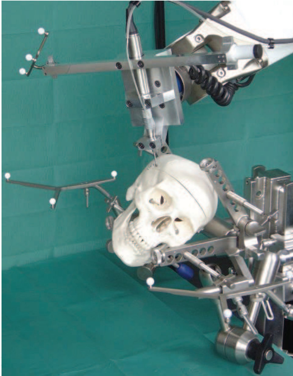
Figure 10. Experimental setup from the RONAF project
