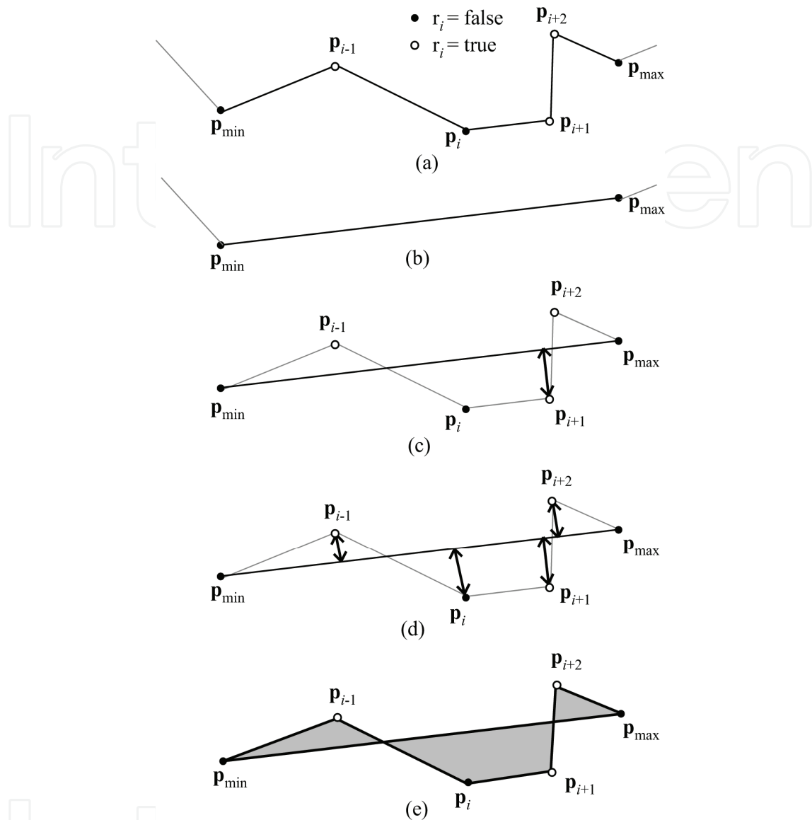
Figure 5. Sketch describing the determination of path deviation d_i . The linear path segments to be compared are the original path (a) and the smoothed path (b). The error functions K_1 , K_2 , and K_3 are illustrated in (c), (d), and (e)
