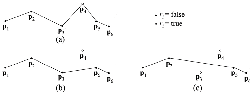
Figure 3. Example for the removal of a path point. Black dots represent still existing path points and white dots represent removed path points. (a) shows the entire path and (b) and (c) the smoothed path before and after removal of p_3 , respectively
