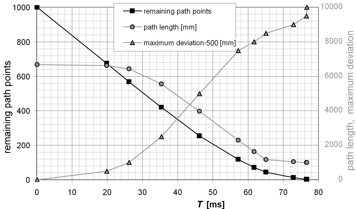
Figure 9. Remaining path points, path length and maximum deviation against computation time T [ms] for the perturbed linear path segment of Figure 8
