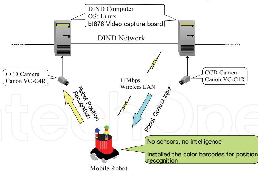
Figure 3. Mobile robot and network system in ISpace
