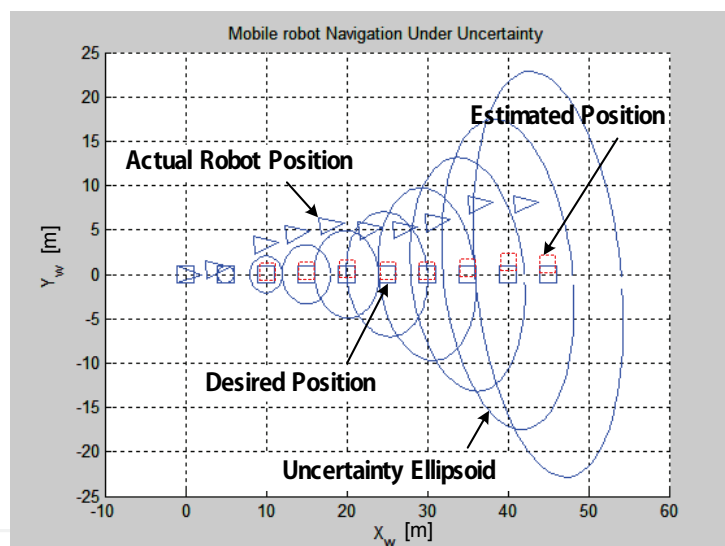
Figure 6. Uncertainty ellipsoids with the movement of a mobile robot
