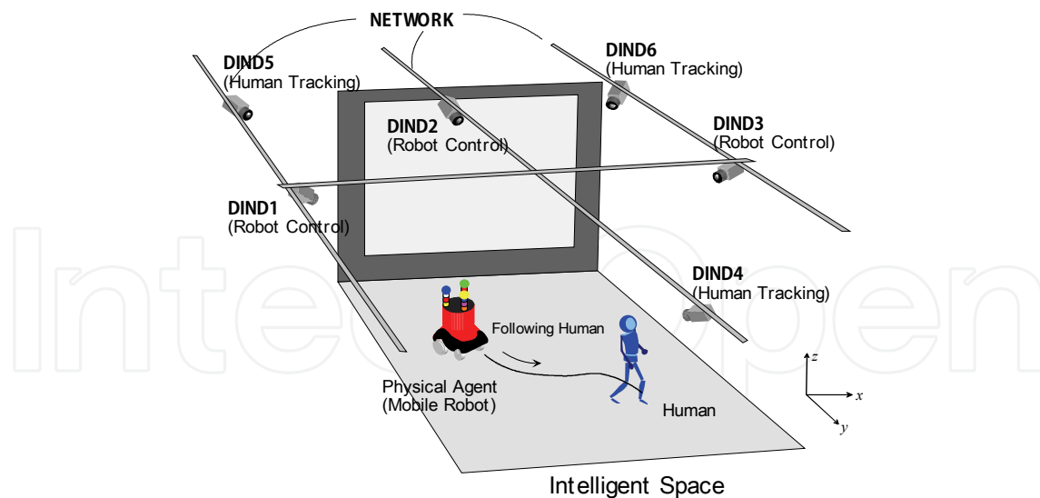
Figure 1. Structure of Intelligent environment by distributed cameras
