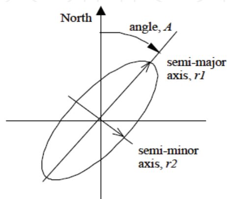
Figure 4. Description of an uncertainty ellipse
