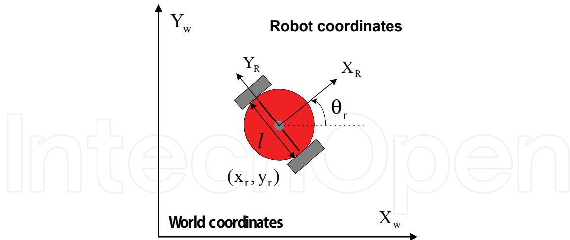
Figure 5. Geometrical model of a mobile robot
