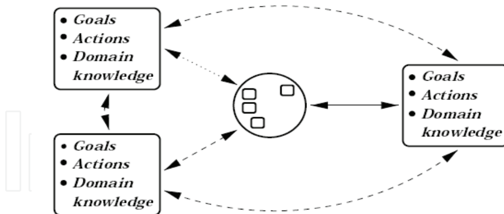
Figure 7. The general communicating MAS scenario. Agents can be heterogeneous to any degree. Information can be transmitted directly among agents as indicated by the arrows between agents. Communication can either be broadcast or transmitted point-to-point (Stone and Veloso, 2000)
