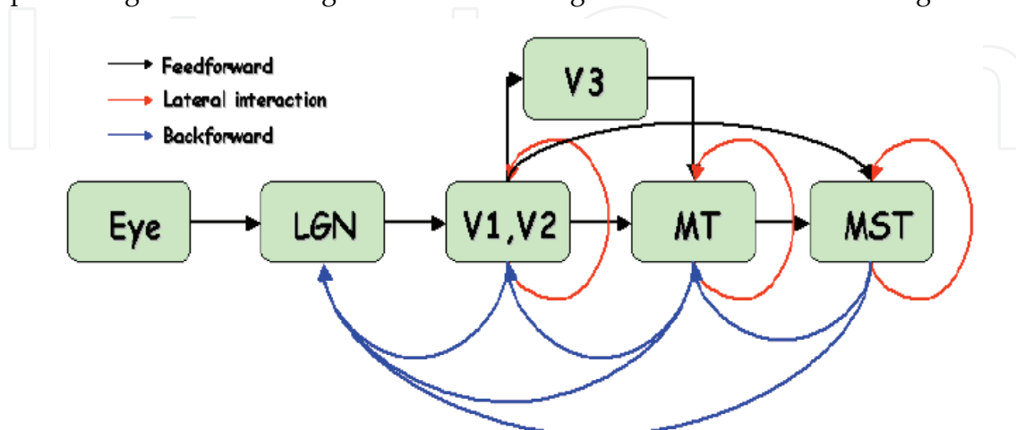
Figure 2. Simplified description of the visual pathway for motion treatment, starting from the eye and ending with the processing in the MST
