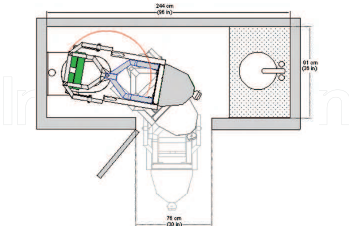
Fig. 9. CAD top view drawing of the HLPR Chair accessing a typical bathroom and toilet. The radius drawn is the area needed for the seat frame to rotate.
