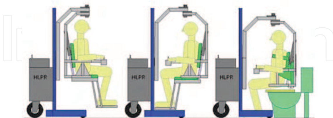
Fig. 7. Graphic showing the concept of placing a patient onto a toilet or chair with the HLPR Chair. The patient drives to the target seat (left), manually rotates near or over the seat (middle) while the torso lifts support the patient and the seat retracts, and then is lowered onto the seat - toilet, chair or bed (right).
