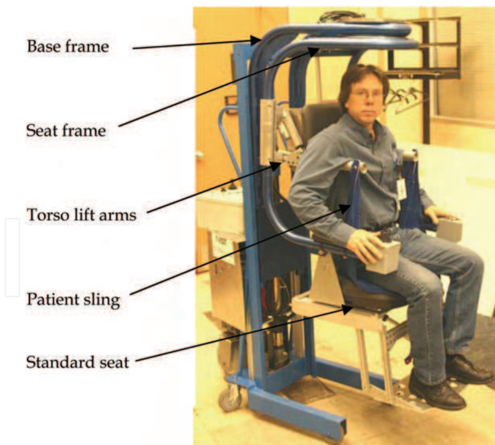
Fig. 13. The modified base and seat frames of the HLPR Chair from the previous welded design.
