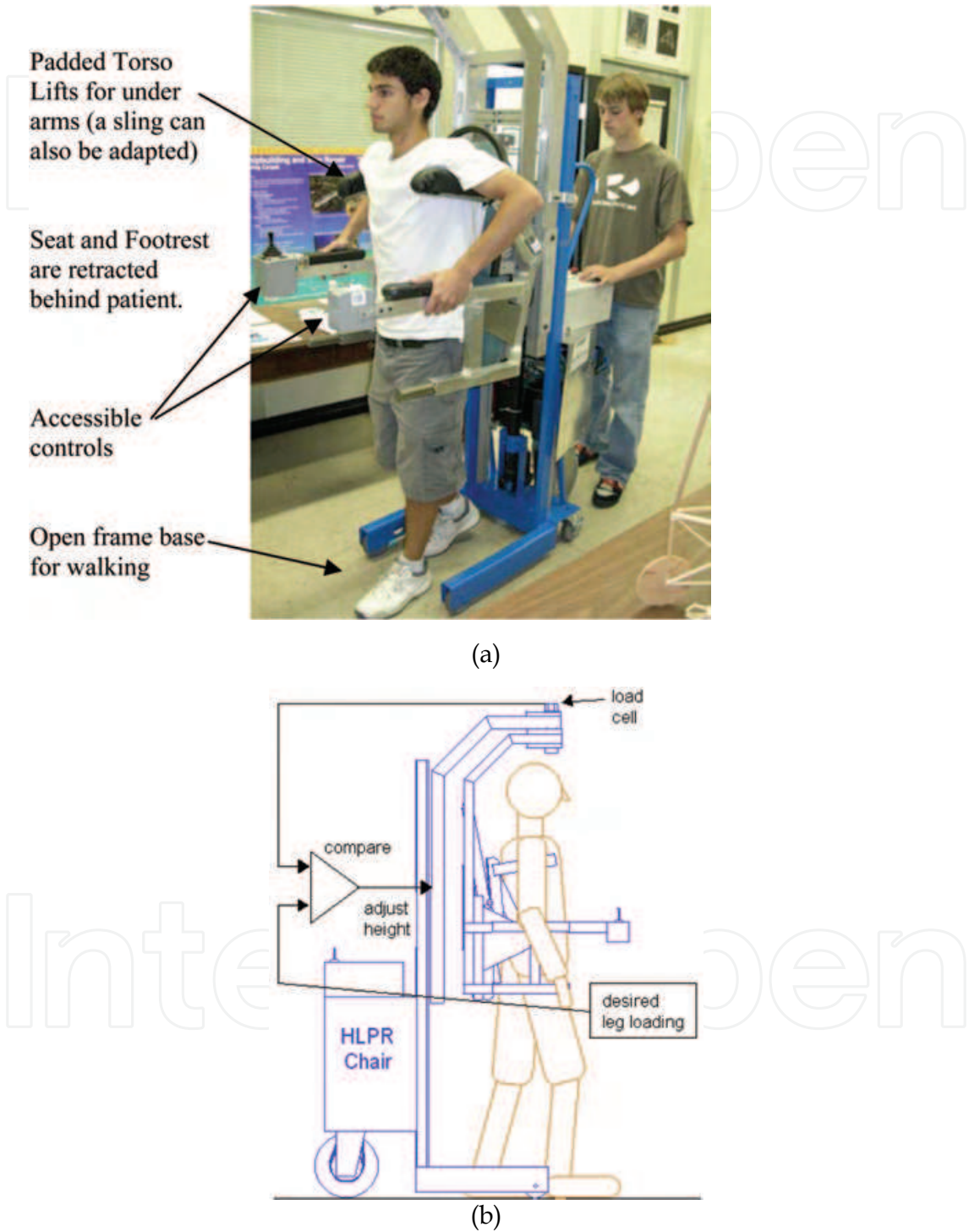
Fig. 12. (a) The HLPR Chair prototype in the rehabilitation/walking configuration. Summer Interns (Alex Page and Robert Vlacich) demonstrate the patient and nurse configuration as part of their official duties. (b) Graphic showing the concept of how the HLPR Chair can be used for patient rehabilitation and incorporate future legs load control.
