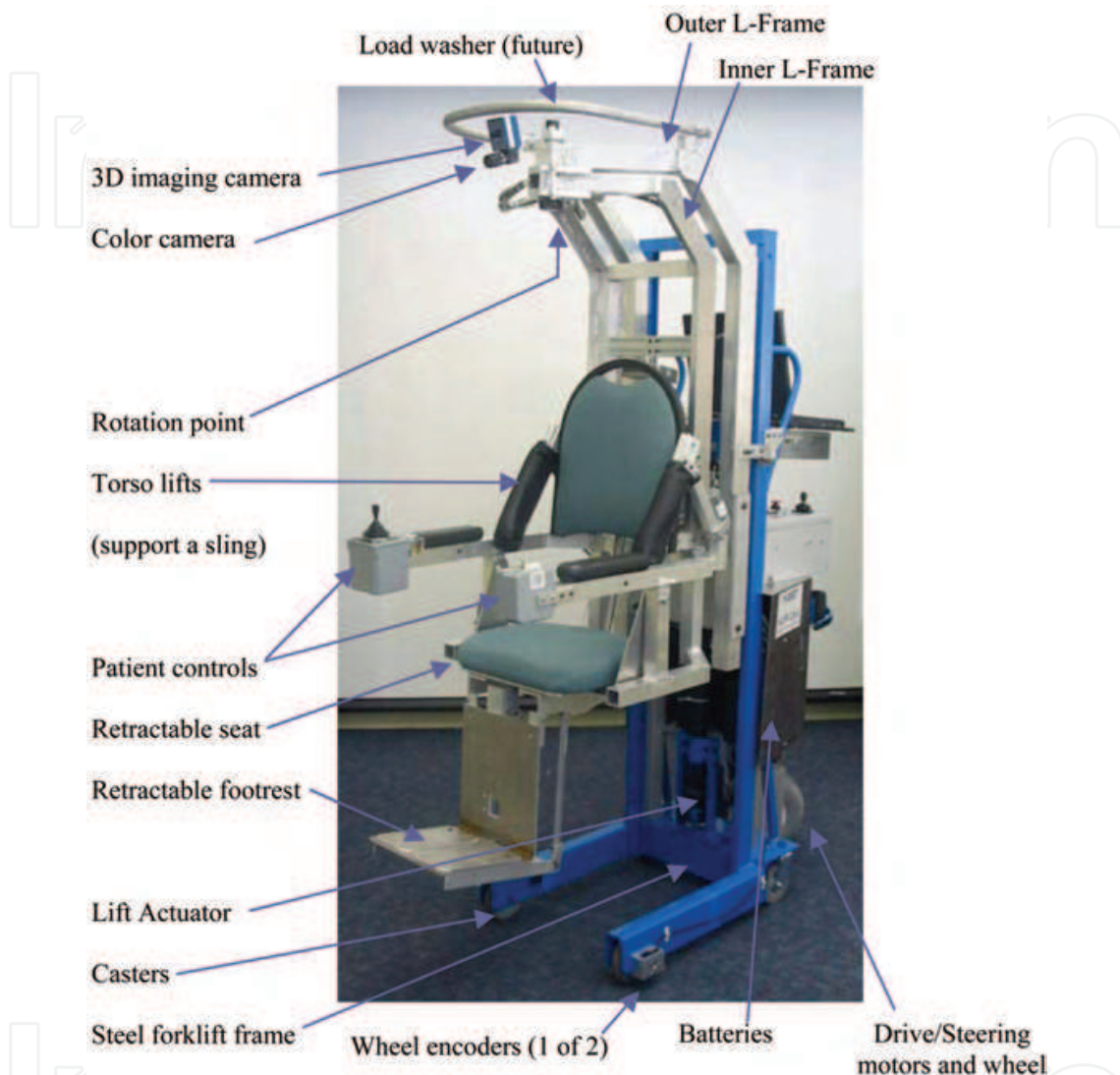
Fig. 5. The HLPR Chair prototype.
