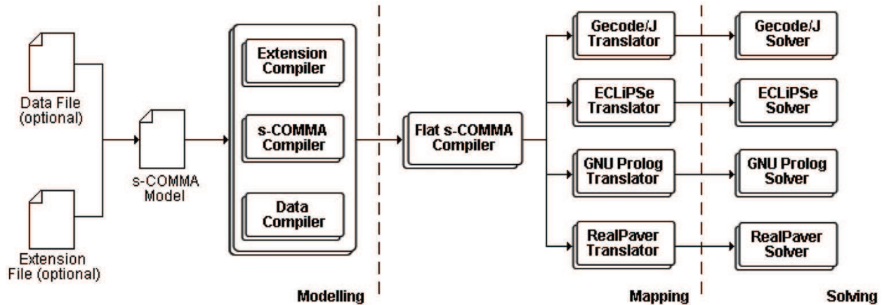
Fig. 7. s-COMMA architecture.
