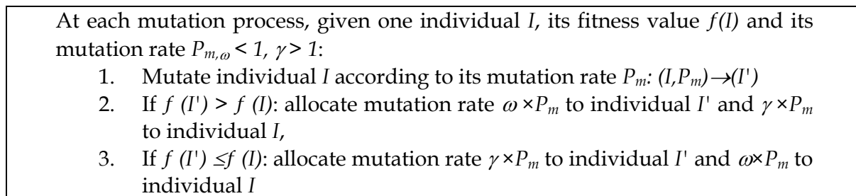
Fig. 4. Basic adaptive mutation rate scheme.
