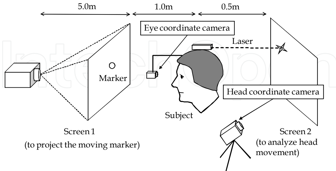
Fig. 2. Experimental setting
