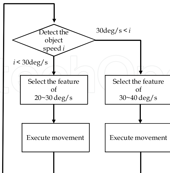
Fig. 11. Implementation model
