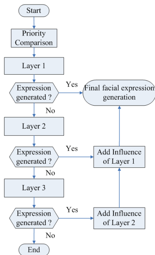
Figure 16. Facial expression generation strategy
