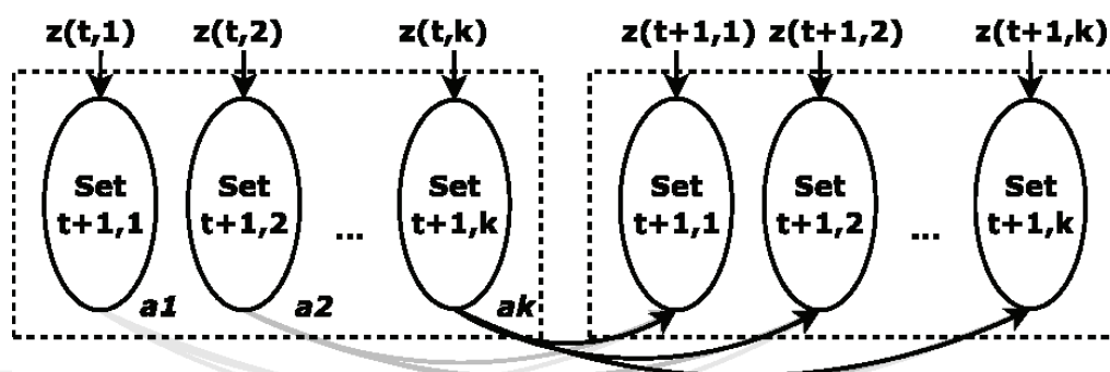
Fig. 1 RTPF operation: samples are distributed in sets, associated with the observations. The distribution is a mixture of the sample sets based on weights \alpha_i (shown as a_i in figure).
