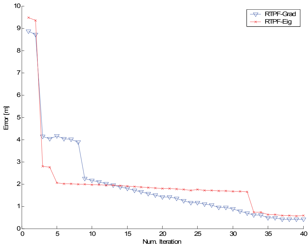
Fig. 6 Performance of the two RTPF versions in the simulated environment of Map 1. The x-axis represents the iterations of the algorithm. The y-axis shows the average error distance of the estimated pose from the actual robot pose.
