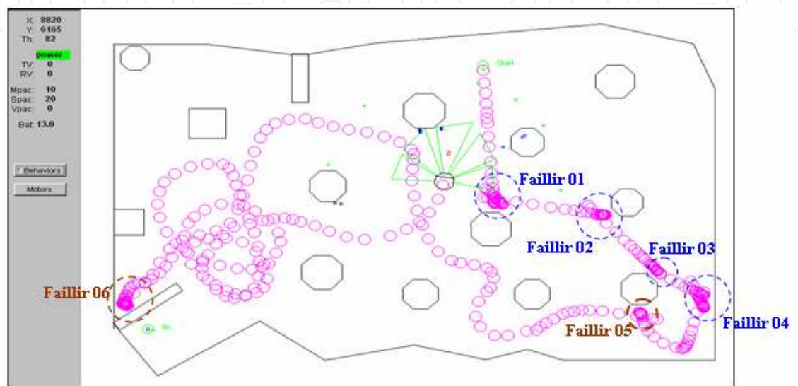
Fig. 30. Trajectories of the robot during the learning of the SIF by algorithm DFQLGA (the first two stages)
