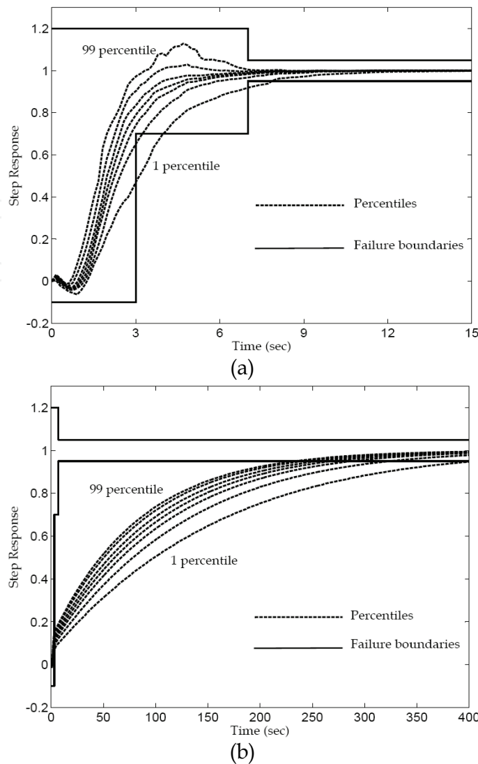
Fig. 8. Step response behaviors of optimum designs (a) point A (b) point C
