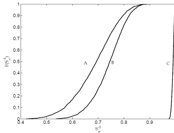
Fig. 14. CDFs for robust stability margins of different optimum designs
