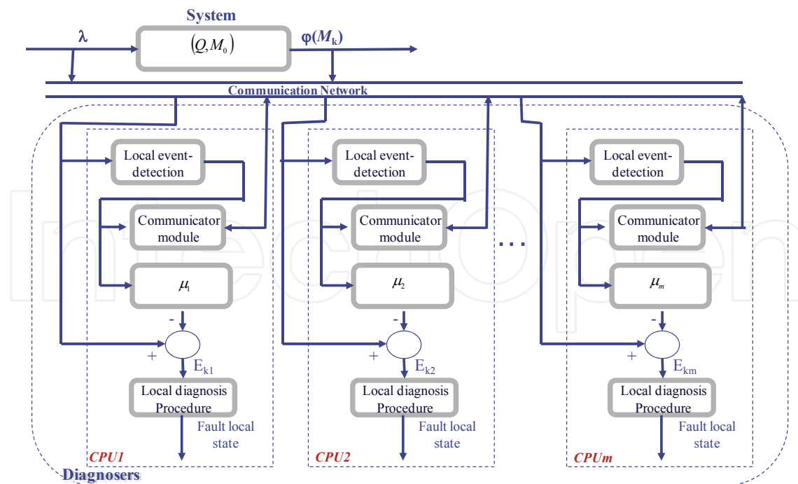
Fig. 9. On-Line Distributed Diagnoser
