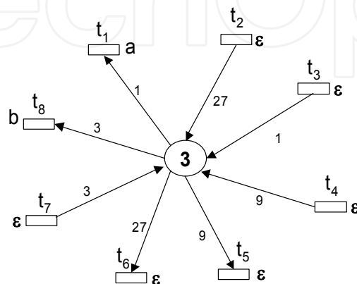
Fig. 7. The IPN reduced diagnoser-model
