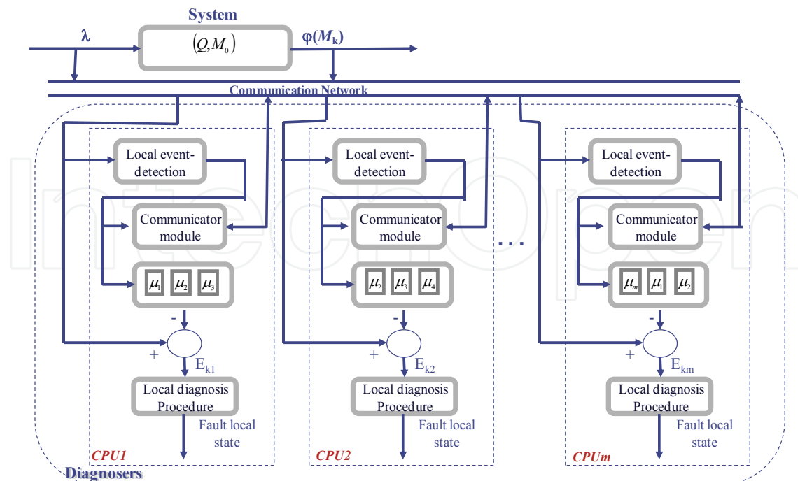
Fig. 10. On-Line Redundant Distributed Diagnoser
