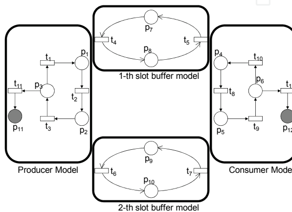
Fig. 2. IPN modules of the identified components
