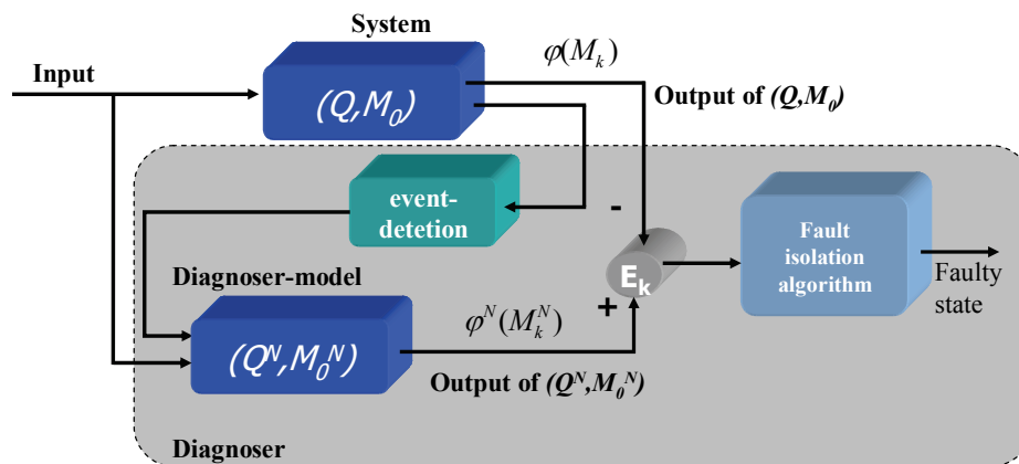
Fig. 5. On-line diagnose scheme
