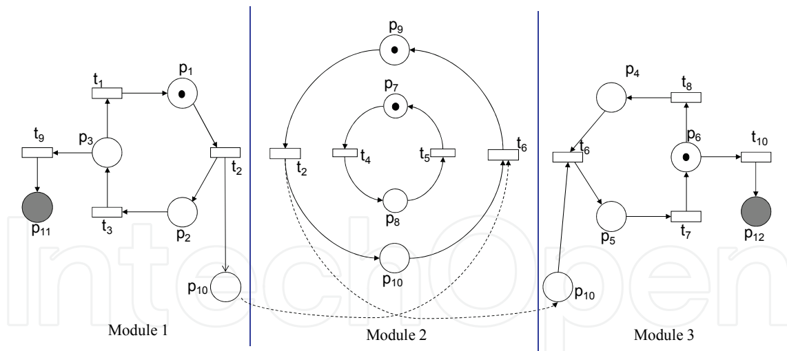
Fig. 8. Distributed Interpreted Petri Net Models
