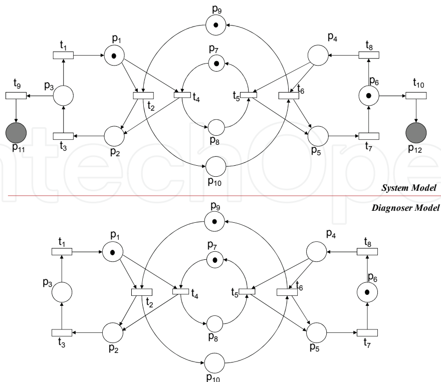
Fig. 6. On-line diagnoser model
