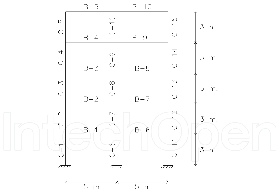
Figure 7. Typical RC building frame of 2 bays and 5 floors.
