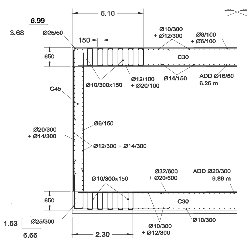
Figure 6. Optimized design of RC box frame.
