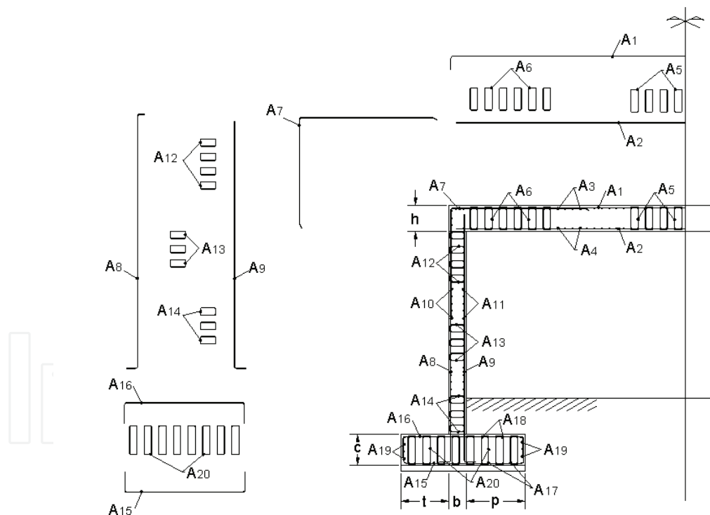
Figure 3. Variables for the RC portal frame.
