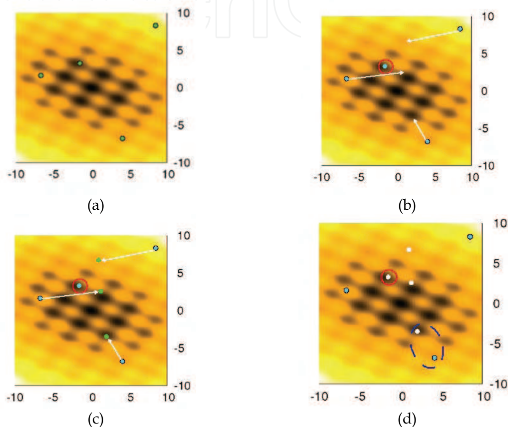
Fig. 5. (a) Create a 'population' of agents (called particles) uniformly distributed over X (feasible region) and Evaluate each particle's position according to the objective function, (b) Update particles' velocities according to equation (5), (c) Move particles to their new positions according to equation (6), (d) If a particle's current position is better than its previous best position, update it.
