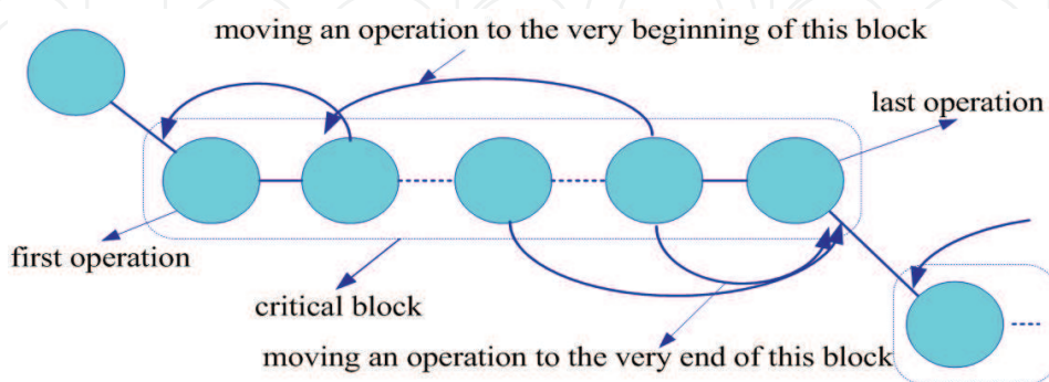
Fig. 4. The N4 neighborhood of moves
