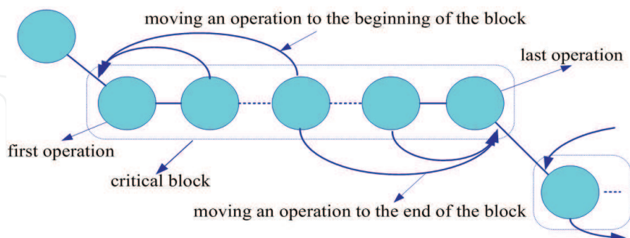
Fig. 6. The N6 neighborhood of moves
