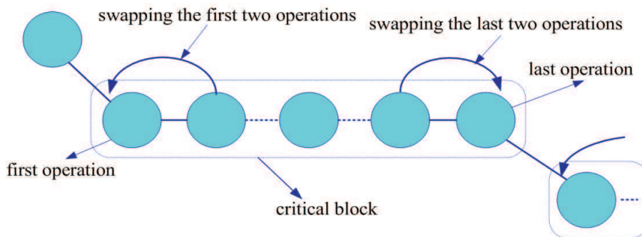
Fig. 5. The N5 neighborhood of moves
