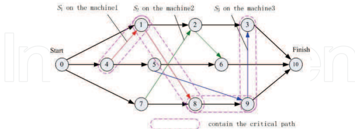
Fig. 2. A feasible solution for the disjunctive graph in Fig. 1
