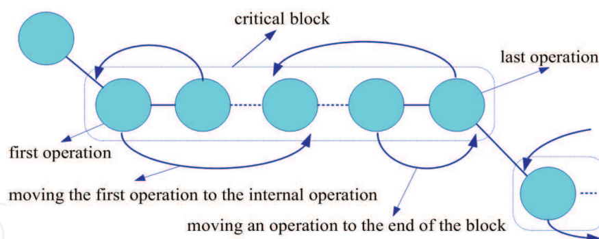
Fig. 7. The further extended neighborhood structure
