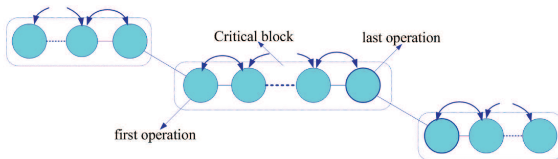
Fig. 3. The N1 neighborhood of moves
