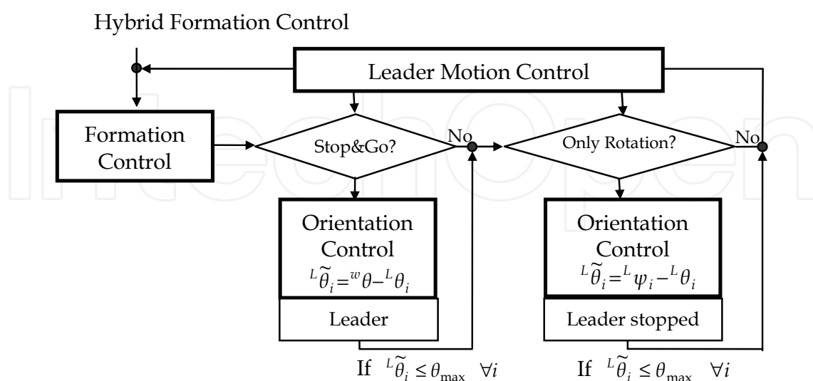
Figure 9. General hybrid formation logic
