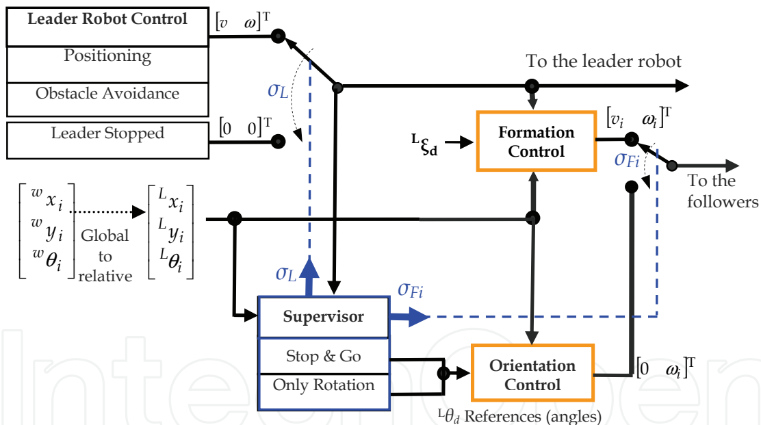
Figure 6. Hybrid formation control block diagram
