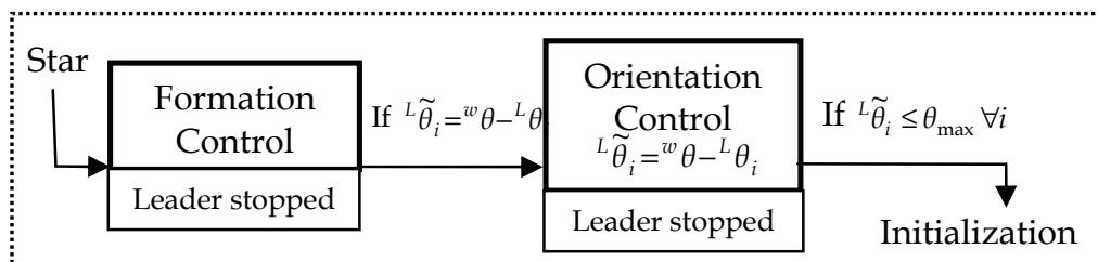
Figure 8. Initialization logic: static formation
