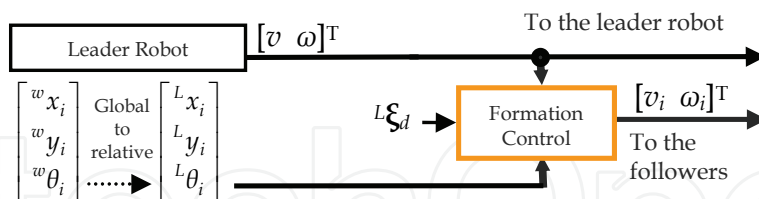
Figure 4. Formation control block diagram
