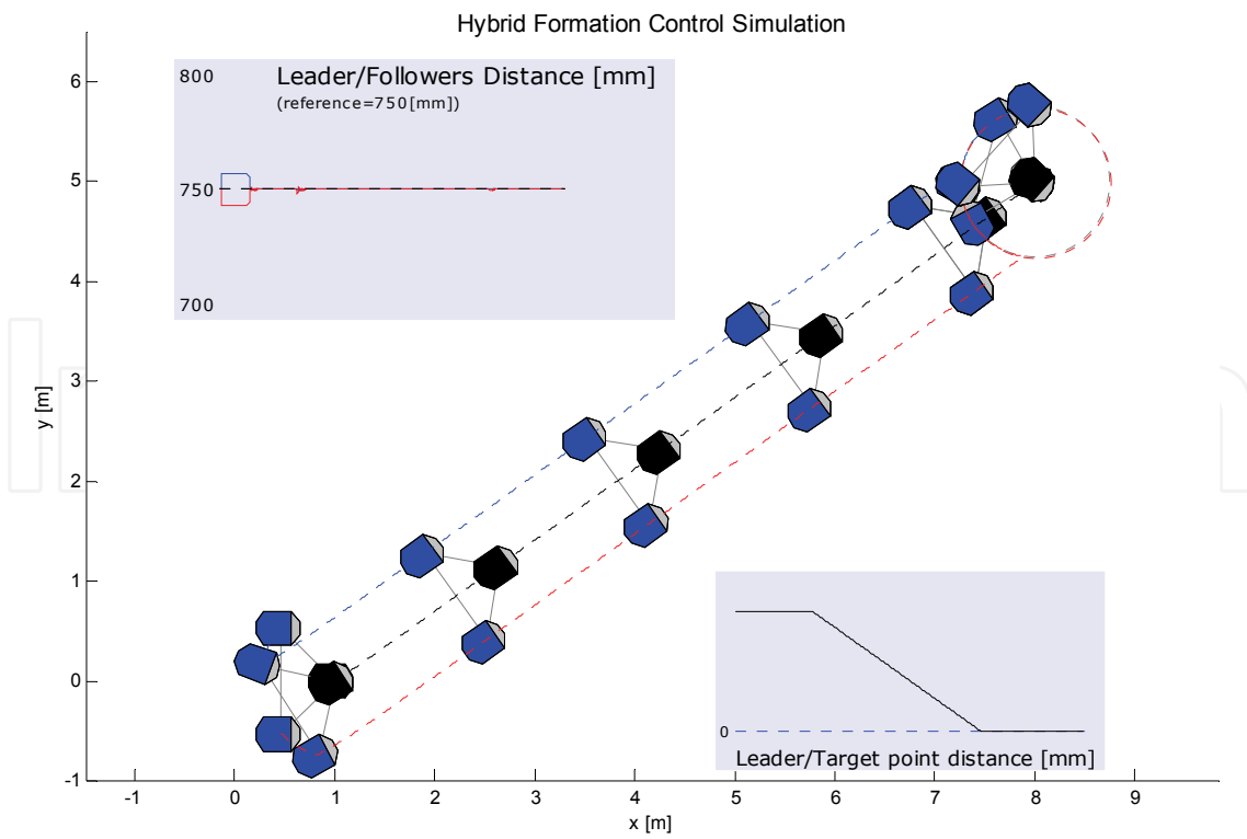
Figure 12. Hybrid formation control simulation
