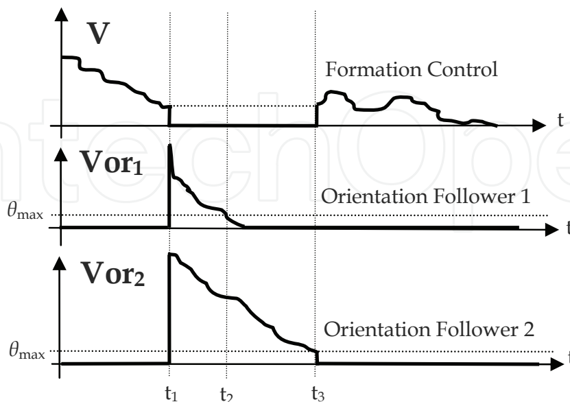
Figure 10. Multiple Lyapunov Function approach
