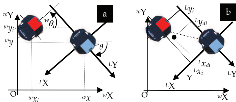
Figure 1. a) Reference systems: world (absolute) reference coordinate system ( O wX wY ), and a second coordinate system attached to the leader robot ( O LX LY ) where the desired positions for each of the followers are defined. b) i -th follower robot positioned at coordinates ({}^L x_i, {}^L y_i) on the leader Cartesian reference where the reference position is given by ({}^L x_{di}, {}^L y_{di})
