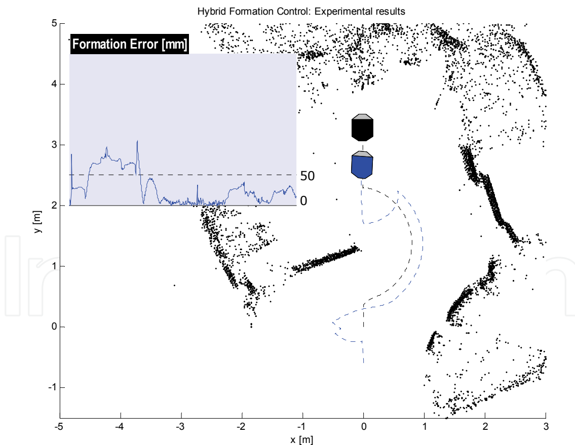
Figure 14. Experimental results: formation control with obstacles
