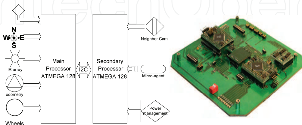
Figure 13. Processing power: block diagram (left), completed board (right)
