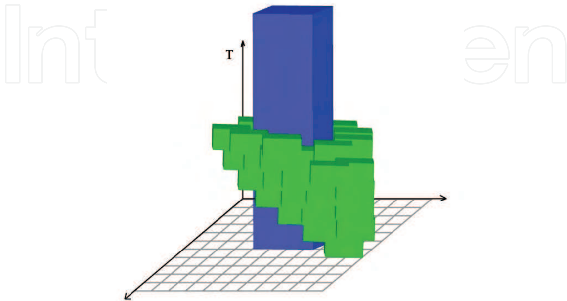
Figure 6. Spacetime Potential bowl growing around a static obstacle
