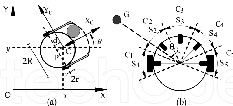
Figure 1. Autonomous mobile robot used in simulations
