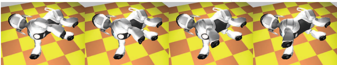
Figure 14: Sequence of the oscillatory movement obtained in simulation for the J1 joint type. The robot is lying on his side to allow the movement of the joint freely. The evolution of the other joint types was performed with the same setup
