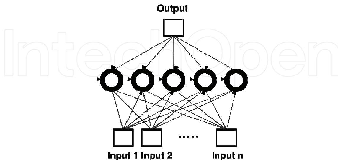
Figure 11. Schematics of the CTRNN used in the walking controller. The hidden units are modeled as leaky integrators
